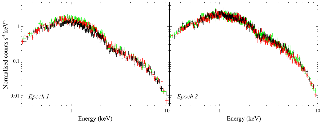
Figure 2. EPIC -pn spectra for the two sets of three observations of Holmberg IX X-1, the first taken in October (left panel; associated with NuSTAR observation 1) and the second in November (right panel; associated with NuSTAR observation 2). The black, red, and green spectra show the first, second, and third observations from each set of three. Although there is some mild flux variability displayed by the observations in each set, it is clear there is very little spectral variability.
