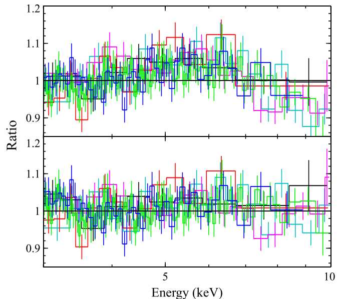
Figure 3. Data/model ratios for the XMM-Newton (black: EPIC -pn, red: EPIC -MOS), Suzaku (green: FI XIS, blue: BI XIS), and NuSTAR (magenta: FPMA, cyan: FPMB) data sets obtained during epoch 1, modeled with both a power-law continuum (top panel) and a bremsstrahlung continuum (bottom panel). The data from the various missions display consistent curvature across their common energy range (3–10 keV). The data have been rebinned for visual clarity.
