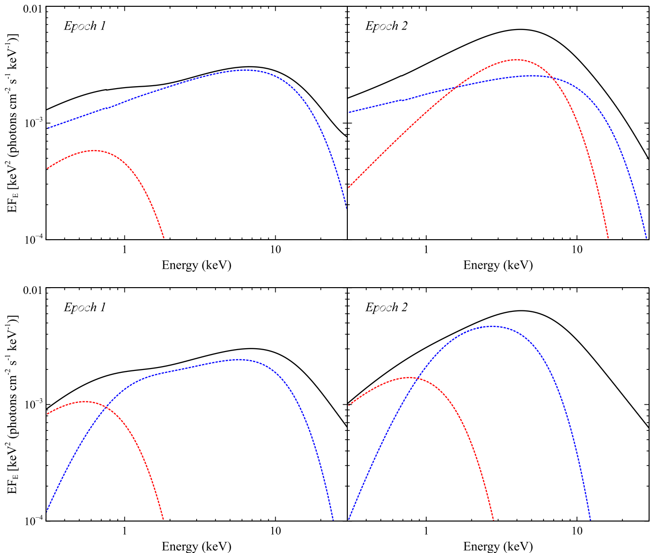
Figure 9. Top panels: the relative contribution of the various spectral components inferred with the DISKBB+SIMPL⊗DISKPBB model (corrected for absorption) for each epoch. The full model is shown in black, while the DISKBB contribution is shown in red, and the DISKPBB contribution (before modification by SIMPL) is shown in blue. In this case, the spectral evolution is dominated by the cooler of the two thermal components (represented by DISKBB). Bottom panels: the same as the top panels, but for the DISKBB+SIMPL⊗COMPTT model. Here, the DISKBB contribution is shown in red, and the COMPTT contribution (before modification by SIMPL) is shown in blue. In this case, the spectral evolution is dominated by the hotter of the two thermal components (represented by COMPTT). (A color version of this figure is available in the online journal.)
