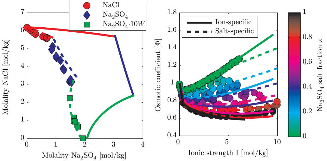
Figure 7.8: Solubility of NaCl, \text{Na}_2\text{SO}_4 , and \text{Na}_2\text{SO}_4 \cdot 10\text{H}_2\text{O} and osmotic coefficient of mixtures of NaCl and \text{Na}_2\text{SO}_4 at 25°C. Data from the CERE Electrolyte Databank [13] Rard et al. (2003)[329]. The aqueous standard state parameters for ions were taken from Table 4.4. The solid NaCl uses \Delta_f G^\circ = -384.14\text{kJ/mol} , \Delta_f H^\circ = -411.15\text{kJ/mol} and C_p = 50.5\text{J/mol/K} , solid \text{Na}_2\text{SO}_4 uses \Delta_f G^\circ = -1270.2\text{kJ/mol} , \Delta_f H^\circ = -1387.1\text{kJ/mol} and C_p = 128.2\text{J/mol/K} , and finally the Glauber salt \text{Na}_2\text{SO}_4 \cdot 10\text{H}_2\text{O} uses \Delta_f G^\circ = -3646.9\text{kJ/mol} , \Delta_f H^\circ = -4327.3\text{kJ/mol} and C_p = 492.2\text{J/mol/K} . Ion indicates that ion-specific parameters from Table 6.11 were used, whereas Salt indicates that the \Delta U_{iw} parameter was fitted to solubility data for the pure salt in water.
