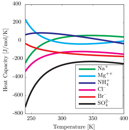
Figure 4.23: Standard state heat capacities as calculated with Eq. (4.61).
