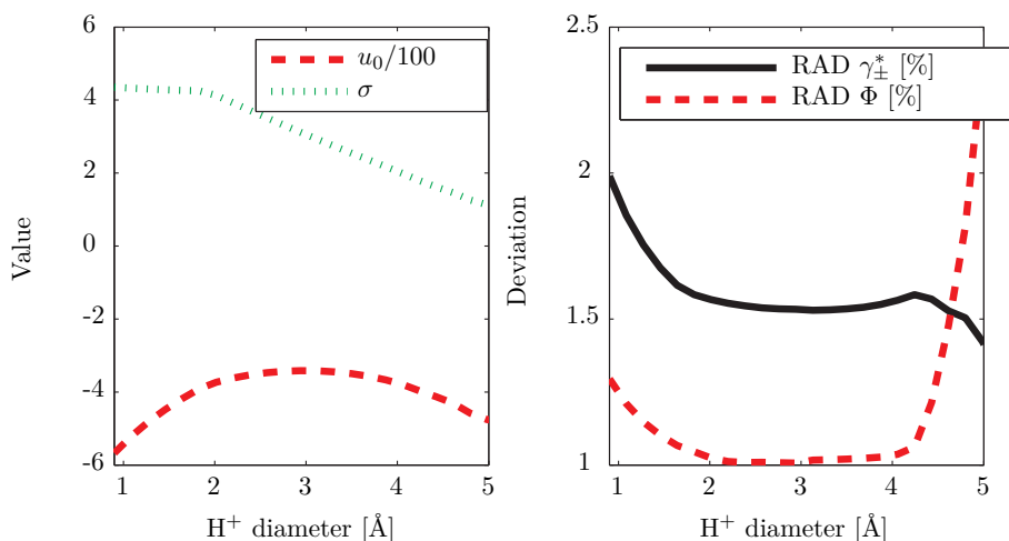
Figure 6.9: Optimized \text{Cl}^- parameters as a function of the \text{H}^+ diameter. Parameters were optimized against experimental activity and osmotic coefficients \gamma_{\pm}^m and \Phi . b_0 parameter was taken from Table 6.1.
