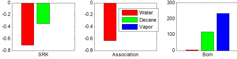
Figure B.6: Contributions to the chemical potential at infinite dilution from different terms.
