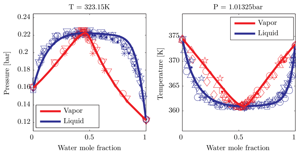
Figure 5.20: P-x,y and T-x,y of the water-1,4-dioxane mixture. Experimental data from the Landolt-Bornstein database [23]. The modeling results were obtained by fitting cross-association parameters \beta_{ij} = 14.88 \cdot 10^{-3} and \epsilon_{ij}/k_B = 1775\text{K} using four negative sites on 1,4-dioxane.
