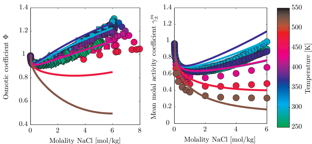
Figure 6.12: T-dependence of Osmotic Coefficient and Activity Coefficients of NaCl with Salt-Specific Parameters. The colored lines are correlations from the e-CPA EoS at different temperatures.
