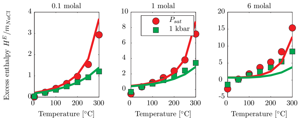
Figure 7.2: Pressure and temperature dependence of excess enthalpy of NaCl in water at 0.1, 1, and 6 molal. Legend applies to all figures.
