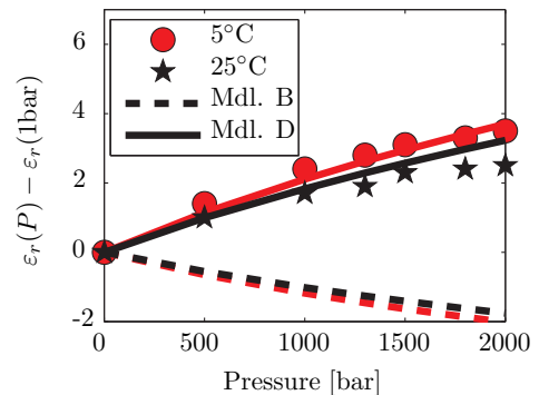
Figure 5.29: Change in static permittivity as a function of pressure at 5°C and 25°C. See model descriptions on p. 107. Experimental data from Potel et al.[320].
