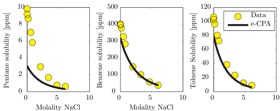
Figure 7.12: Solubility of pentane, benzene, and toluene in Water+NaCl at 25°C. Data from Price (1976) [340].
