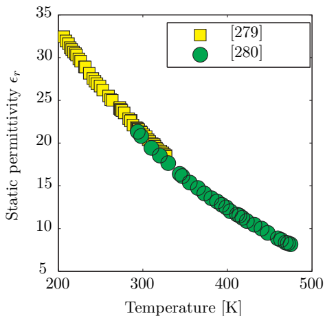
Figure 5.12: Static permittivity of acetone and comparison to experimental data from Cole (1941) [279] and Teutenberg (2009) [280]
