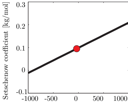
Figure 7.9: The effect of \Delta U_{SG} (solid line) on k_S for \text{CO}_2 in NaCl and exp. k_s = 0.095\text{kg/mol} .
