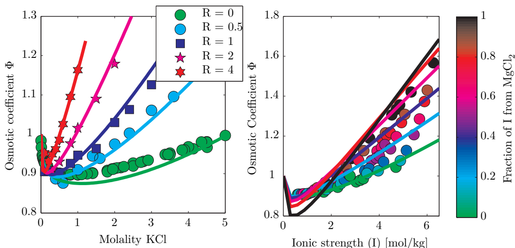
Figure 7.5: Osmotic coefficients in aqueous solution of KCl+NaCl (left) with R = m_{\text{NaCl}}/m_{\text{KCl}} and KCl+NaCl+MgCl 2 (right) of mixtures of Water+KCl+NaCl+MgCl at 25°C and R = 0.752 . Data from [325].
