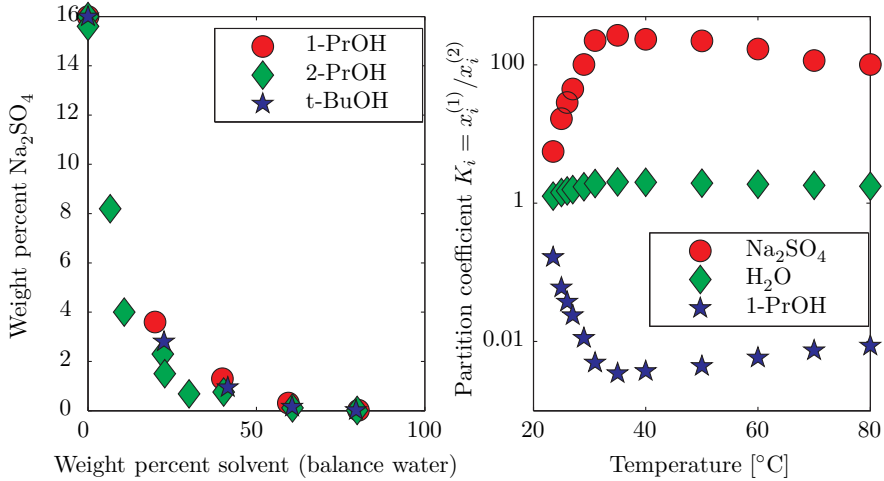
Figure 1.10: Solubility of salts in mixed solvents at 20 °C (left) (PrOH = propanol, BuOH = butanol) (left) and distribution of compounds in the Na 2 SO 4 -H 2 O-1-propanol system at salt saturation (right). Data from [44].
