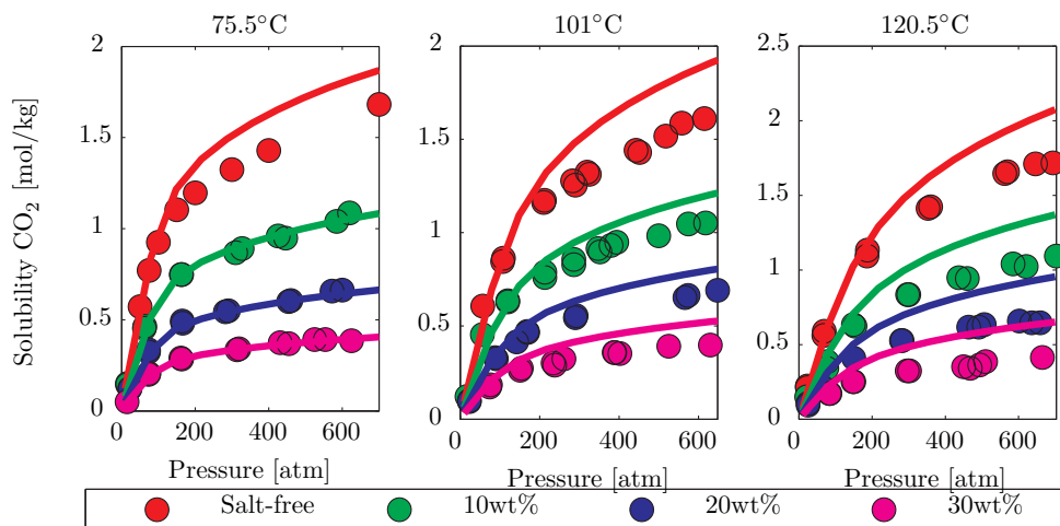
Figure 7.11: Predicted solubility of CO 2 in Water+CaCl 2 . Data from Prutton and Savage (1945) [338] and Wiebe and Gaddy (1940) [339].
