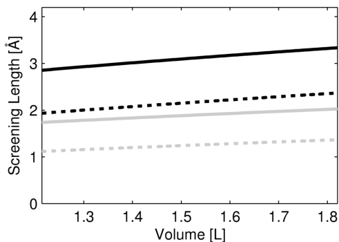
Figure 4.7: Effect of volume on the screening length calculated by MSA (solid) and Debye-Hückel (dashed) for NaCl (black) and \text{MgCl}_2 (gray) at 25^\circ\text{C} , 3 molal, and relative static permittivity \epsilon_r=78 .
