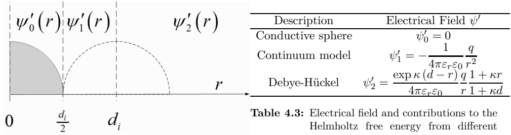
Figure 4.19: Electrical field in the vicinity of an ion with diameter d_i .
