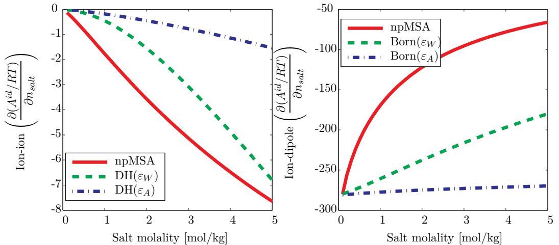
Figure 4.28: Chemical potential of salt and solvent from Non-primitive MSA and Born. DH( \epsilon_X ) or Born( \epsilon_X ) indicates whether the Wertheim static permittivity \epsilon_W from Eq. (4.84) or the Adelman A from Eq. (4.85) was used in the model.
