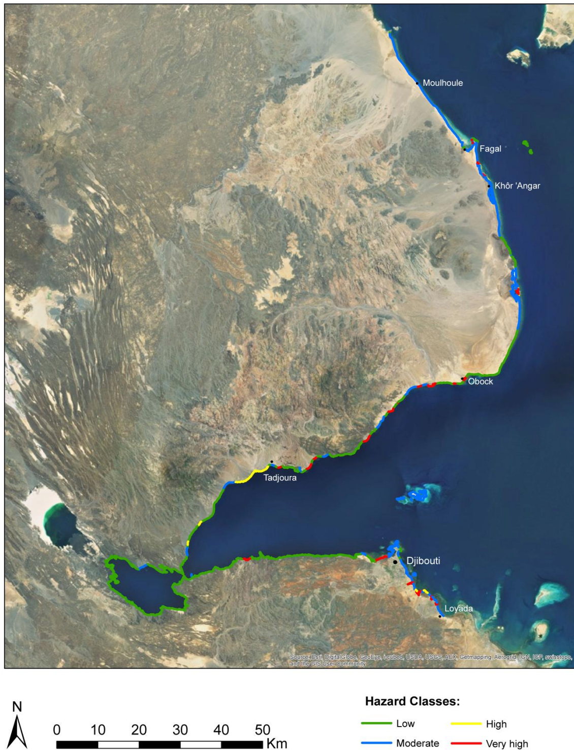
Fig 6. National hazard map for flooding
