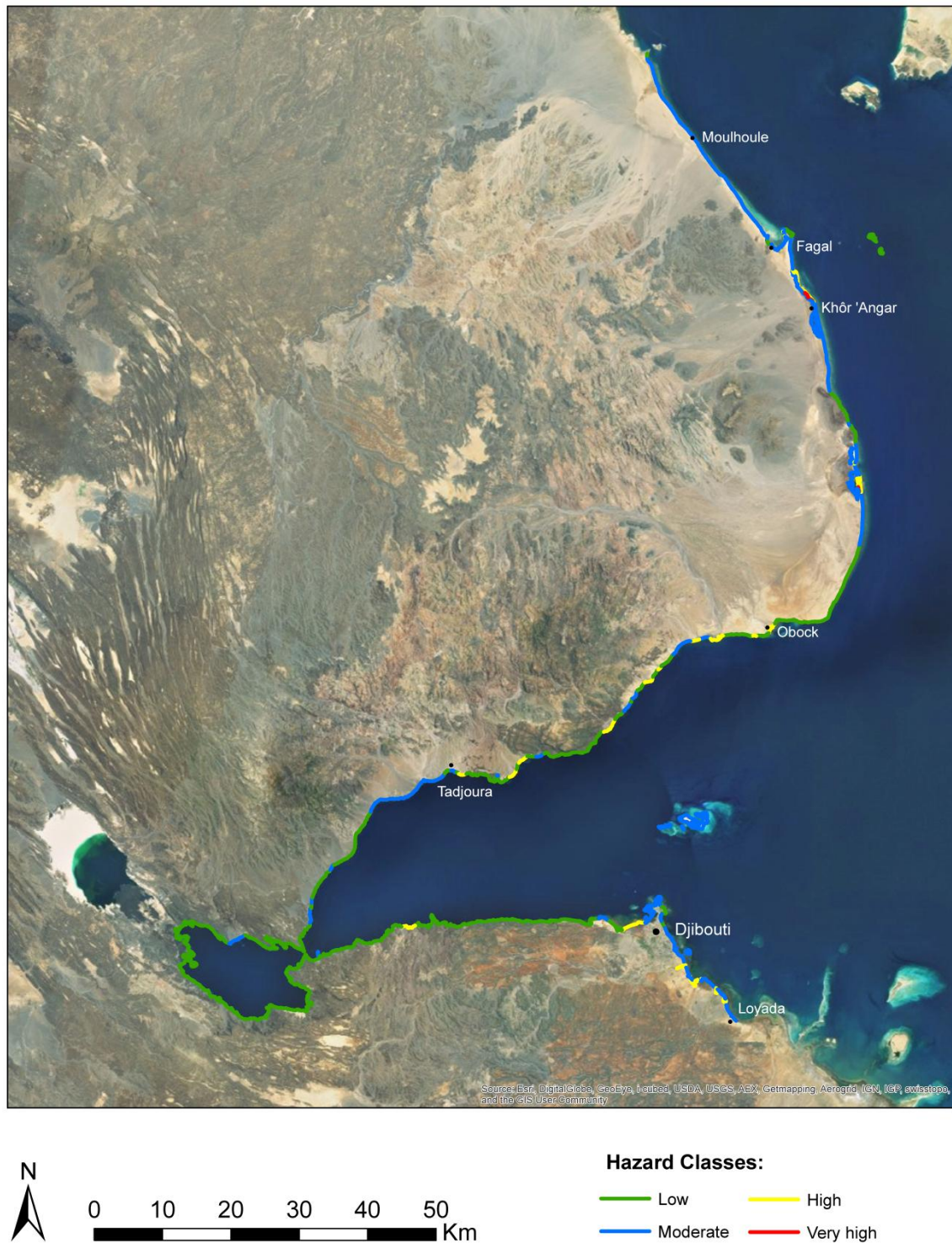
Fig 4. National hazard map for salt water intrusion
