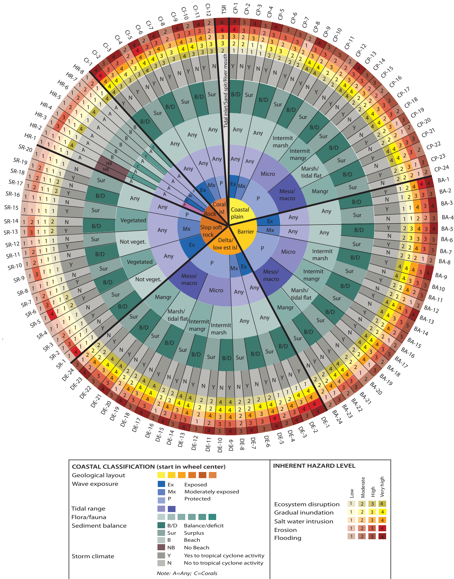
Fig 1. The Coastal Hazard Wheel (Rosendahl Appelquist 2012).
