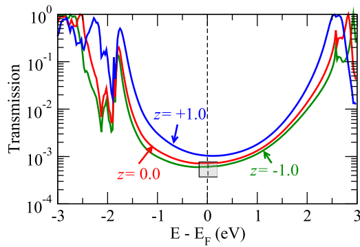
FIG. 8. (Color online) The transmission function for the zero-stress Au/B4APA junction configuration ( S_0 ) calculated from the DFT+ \Sigma method using three different image plane positions, namely z = +1.0, -1 Å relative to the Au tip atom. The gray box indicates the experimental conductance 0.57 \pm 0.2 ( 10^{-3}G_0 ), and the Fermi level indicated by the dashed line is set to 0 eV [15].
