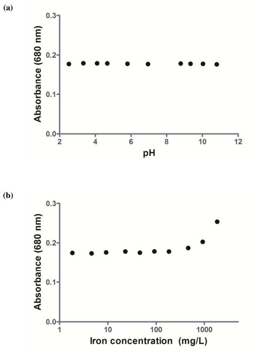
Figure S3. Effect of pH and residual iron ions concentration on phenol determination (added phenol concentration = 20 \mu M)
