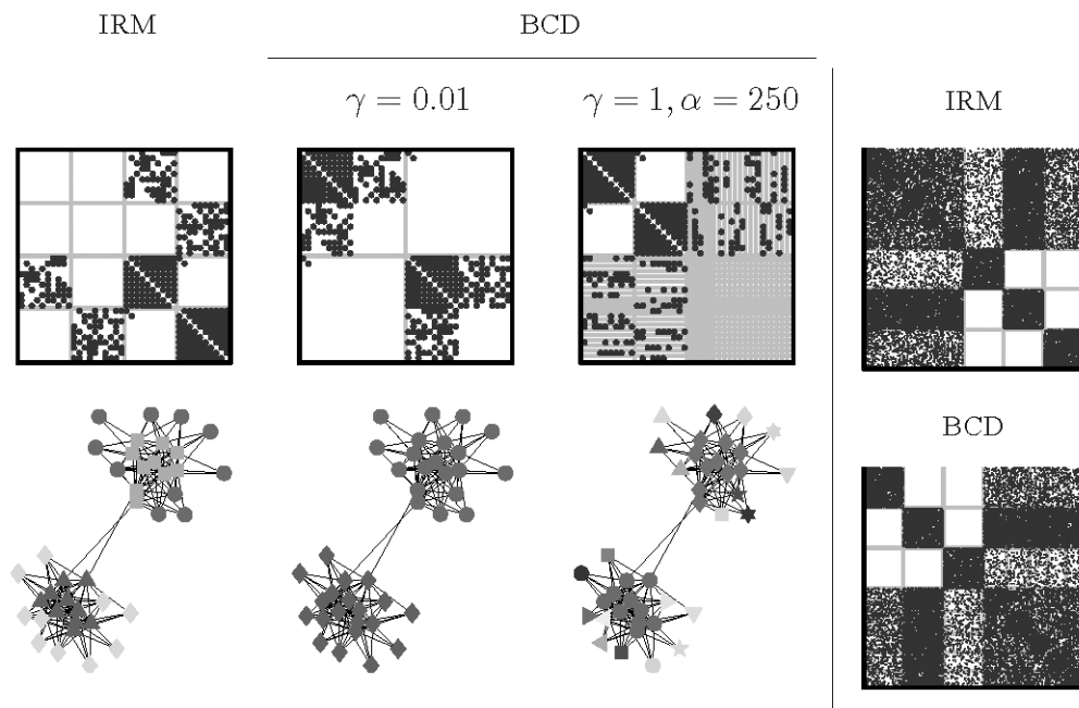
Figure 2: Left: IRM and BCD analysis of a synthetically generated network of 40 nodes with two groups of 20 nodes each subdivided into ten nodes forming a core and ten nodes defining the periphery (i.e. satellite communities). Right: IRM and BCD analysis of synthetically generated network with five smaller and three larger communities.
