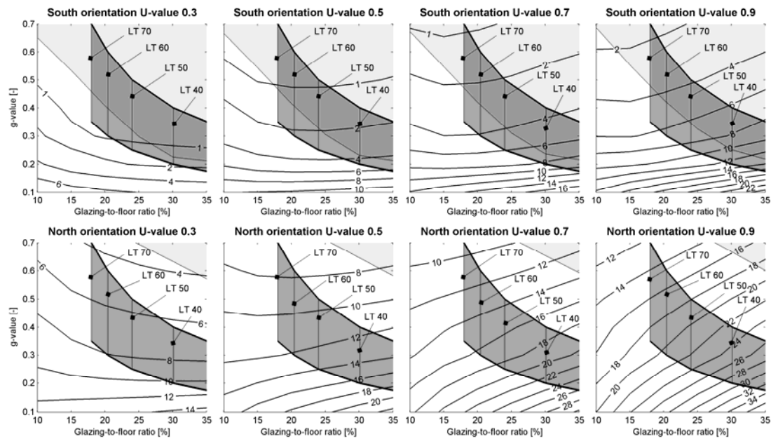
Figure 10: Contour plots of space heating demand for various g -values and glazing-to-floor ratios, indicating overheating and the specified daylight target for a room with dimensions of 4\text{m} \times 4\text{m} and for various glazing U -values.
