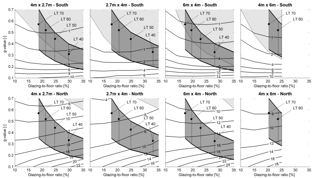
Figure 4: Contour plot of space heating demand for various g-values and glazing-to-floor ratios, indicating overheating and the specified daylight target for two different room sizes with a width-to-depth ratio of 1:1.5 and 1.5:1 and for a glazing U-value of 0.5 W/m 2 K.
