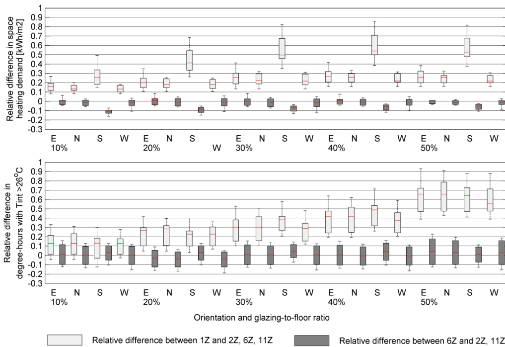
Figure 8: Comparison of space heating demand and degree-hours with indoor temperature > 26^{\circ}\text{C} for different thermal zone configurations with different glazing-to-floor ratios and orientations.
