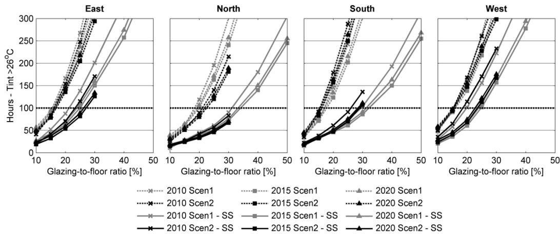
Figure 4: Hours with indoor temperatures > 26^{\circ}\text{C} for different orientations and glazing-to-floor ratios and a scenario with and without dynamically controlled solar shading.
