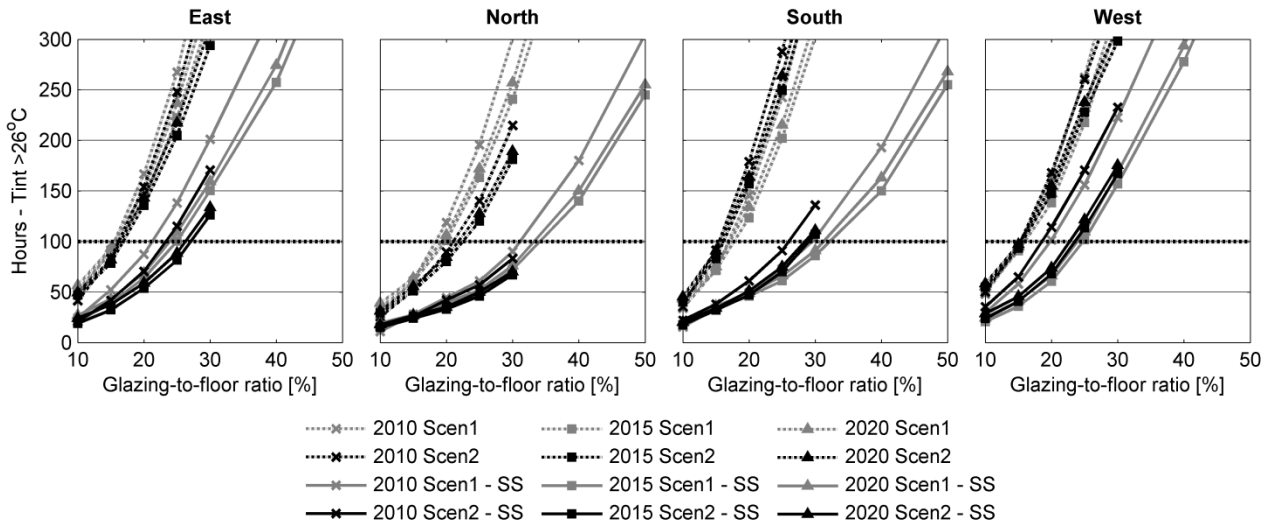
Figure 5: Hours with indoor temperature > 26°C for different orientations and glazing-to-floor ratios.
