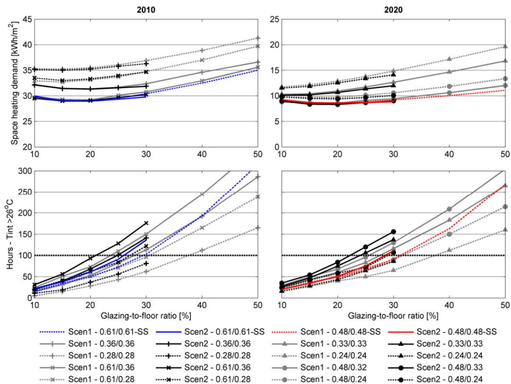
Figure 6: Space heating demand and hours with indoor temperatures > 26^{\circ}\text{C} for different glazing types and glazing-to-floor ratios for the south orientation of the house.
