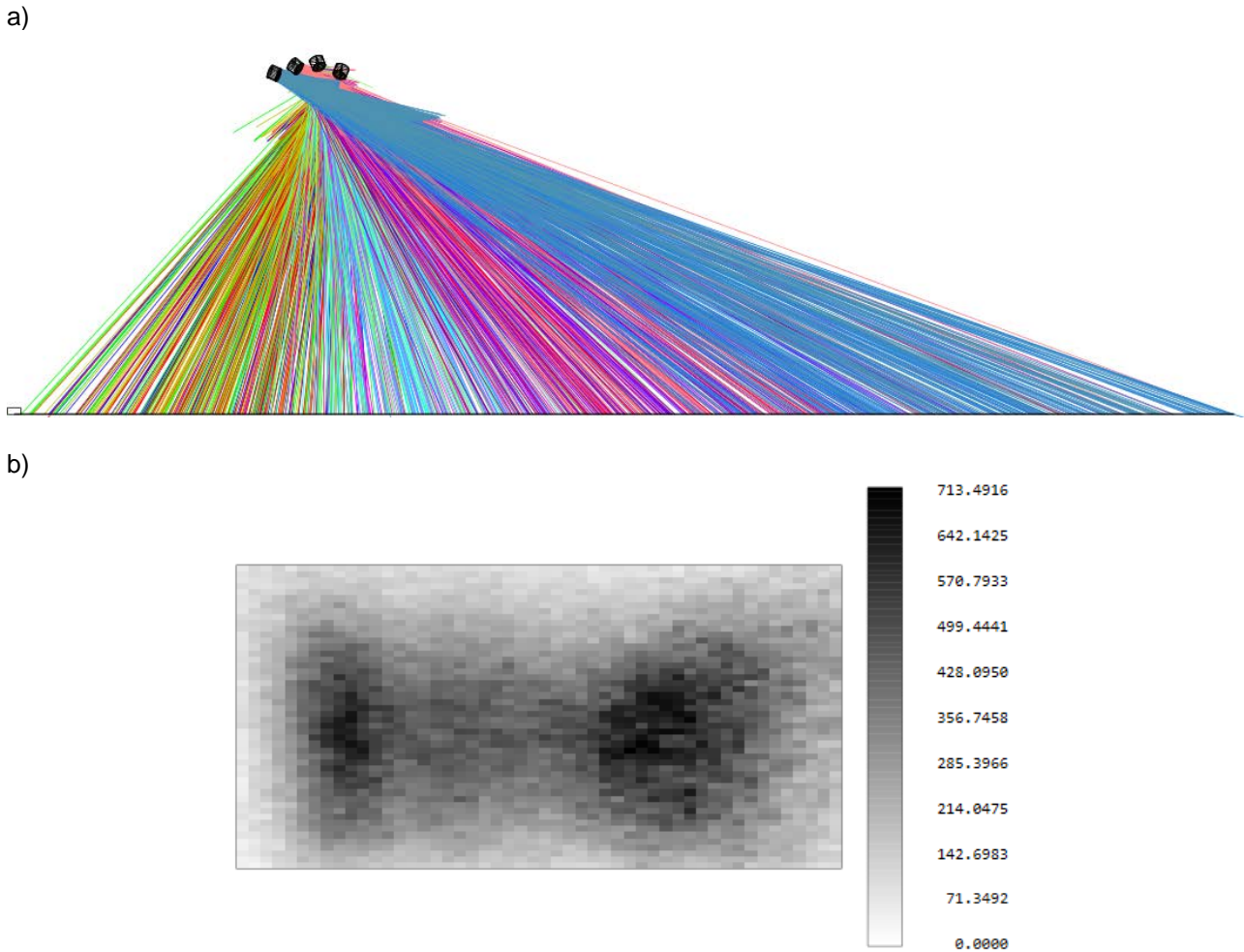
Figure 1. Visualization of the ray tracing of the lighting mock-up different LEDs have differently colored rays a). Simulated illuminance distribution on task from symmetric lenses b).
