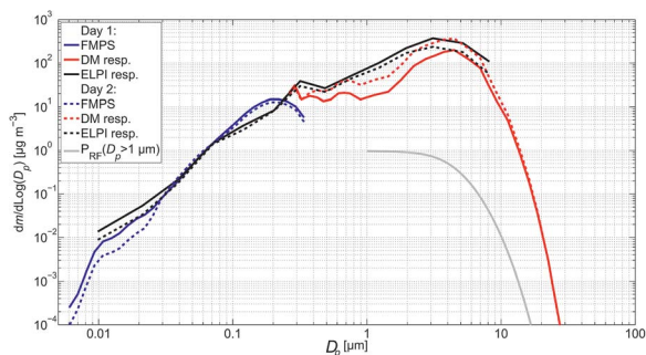
Fig. 4 Respirable mass distribution averages calculated over the gravimetric NF sampling period and P_{\text{RF}} shows the simplified respirable fraction penetration efficiency for particles over 1 µm in diameter.
