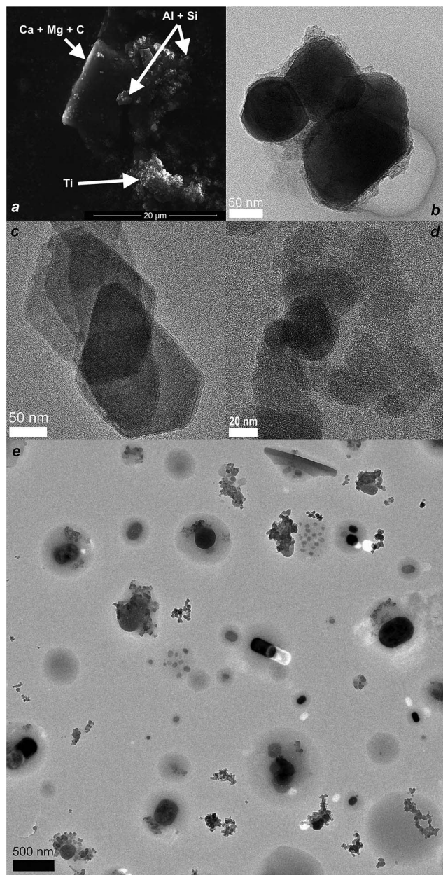
Fig. 7 Micrographs of collected particles: (a) SE image showing dolomite (Ca + Mg + C), mica (Al + Si) and TiO 2 (Ti) particles and HRTEM images of (b) agglomerated TiO 2 , (c) mica sheets, (d) soot, and (e) overview of mixed particles.
