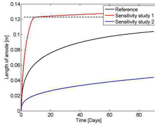
Figure 6.18 Length of anode as a function of the exposure time, for the three sensitivity studies.
