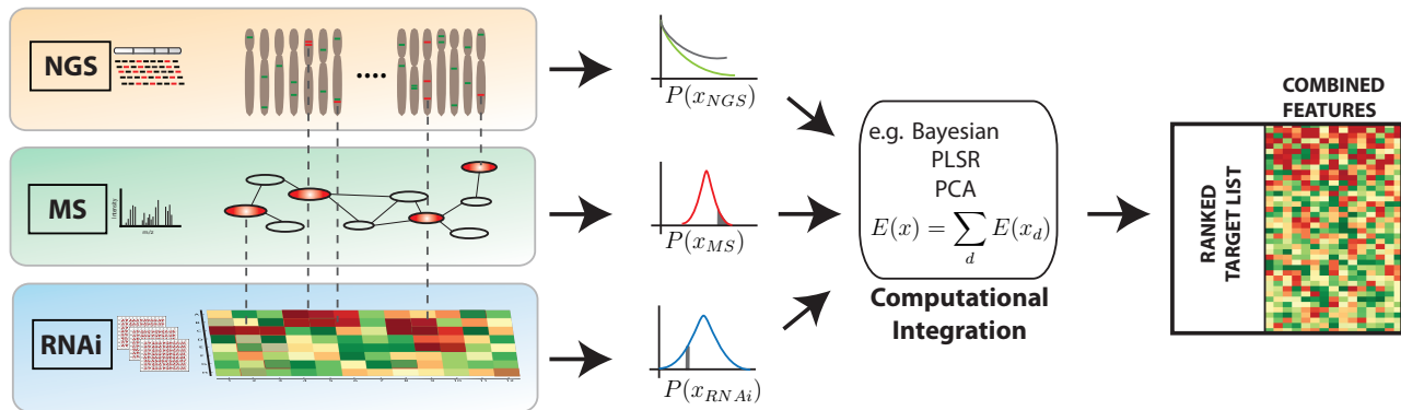
Figure 6 - Conceptual workflow for conducting integrative network biology experiments. By interrogating a biological system from the genome (NGS), global proteome (MS) and phenotype (RNAi) perspective, we can systematically assess the role of particular gene mutations and proteins in a given disease. Through computational integration of these datasets in an un-biased manner, potential targets can be ranked based on the amount of evidence that is highlighting their importance.
