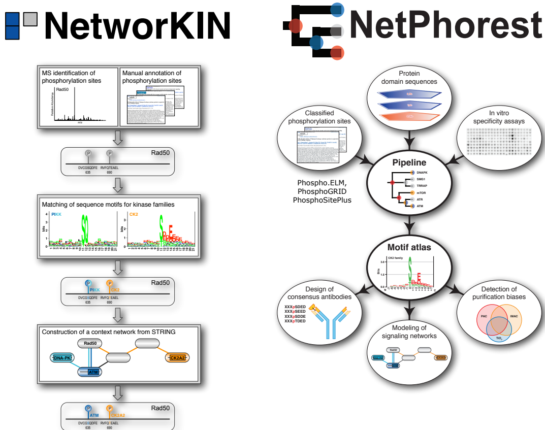
Figure 5 - Overview of the NetworkKIN and NetPhorest workflows. By integrating motif-level predictions originating from Netphorest with protein contextual information from STRING, NetworkKIN allows prediction of in vivo kinase-substrate interactions based on experimentally observed phosphorylation sites 98,162,163 .
