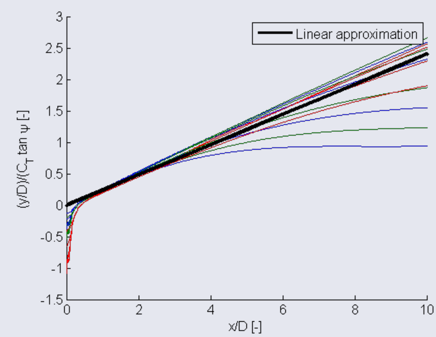
Figure 4: Normalized wake path function.
