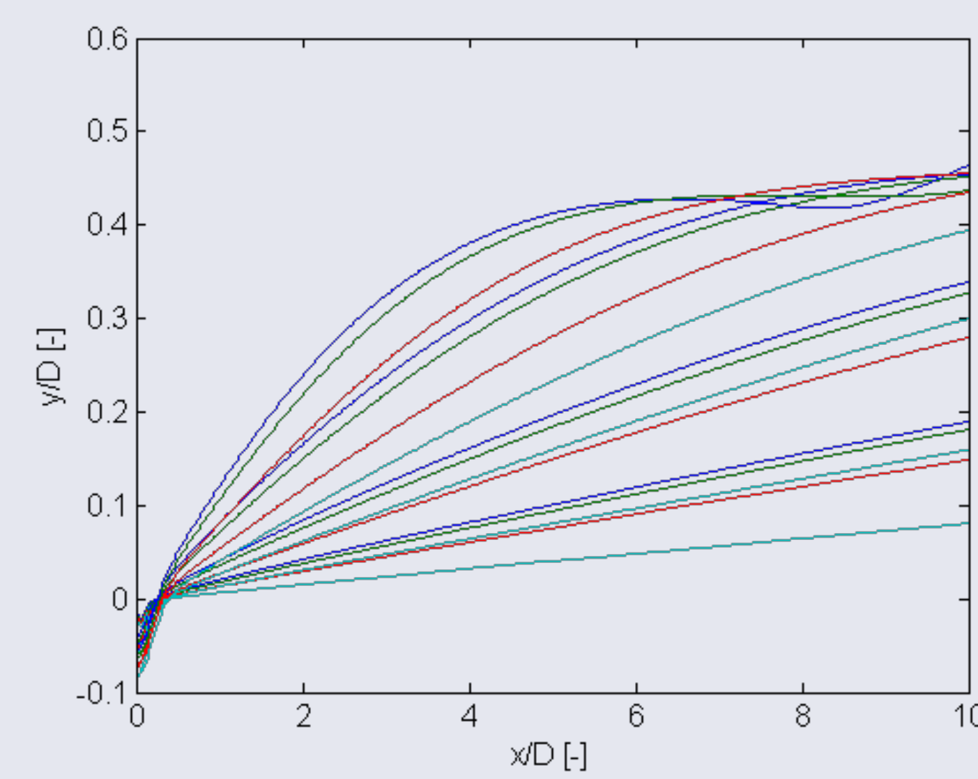
Figure 3: Wake path function plotted for all values of C_T and \psi .
