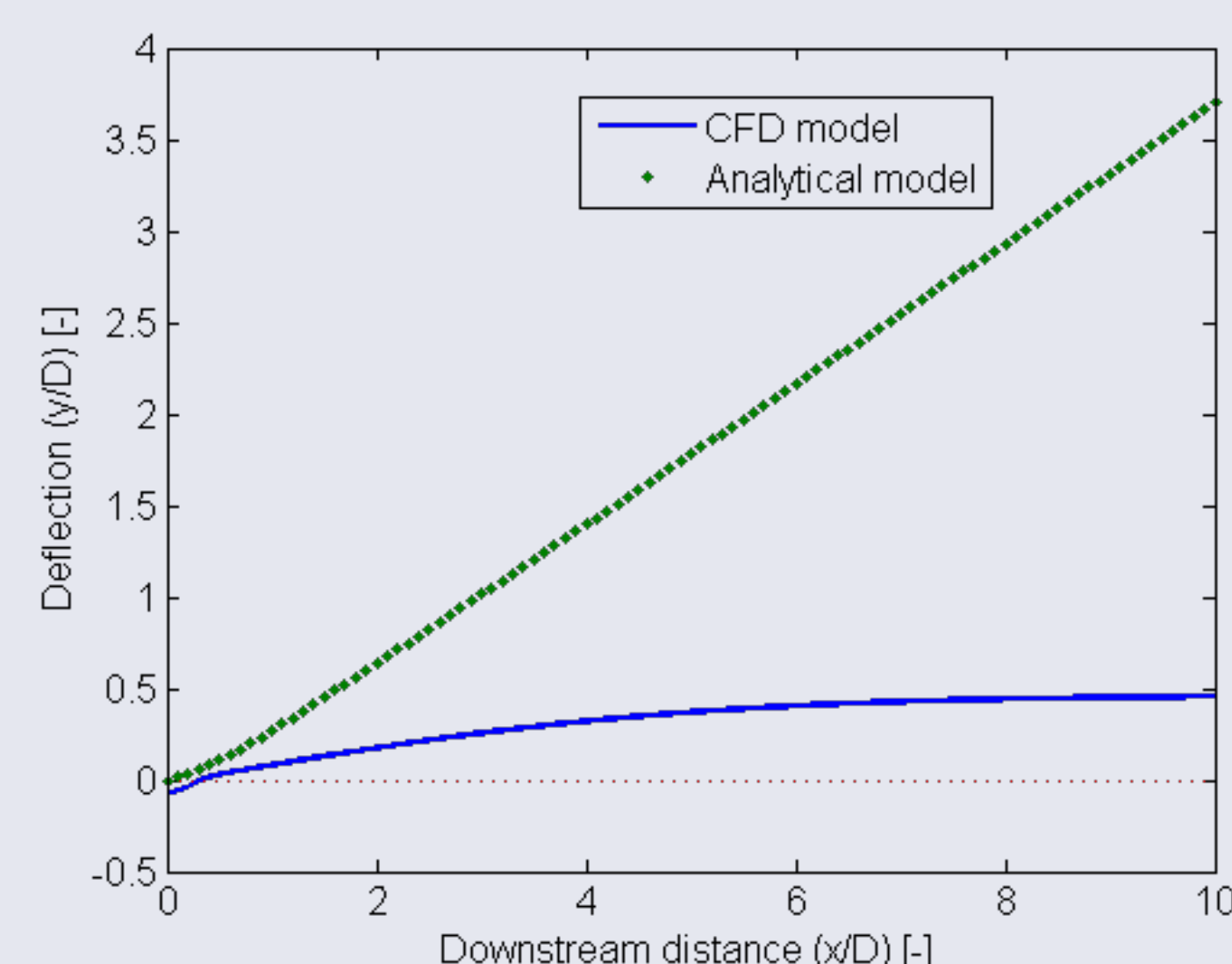
Figure 2: Comparison between the analytical model and CFD data for a test case of C_T = 0.64 , \psi = 30^\circ .
