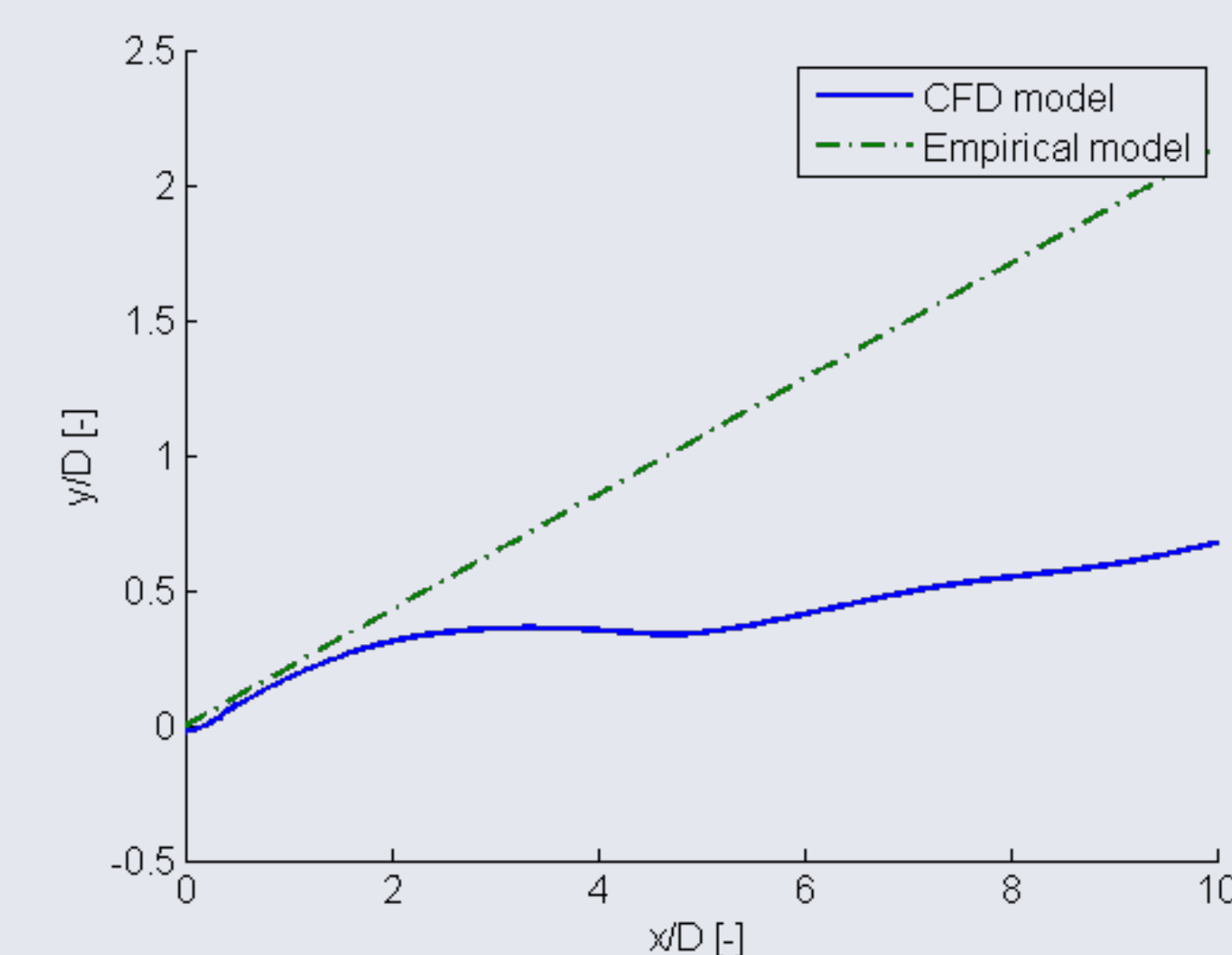
Figure 8: C_T = 0.89 , \psi = 45^\circ .
