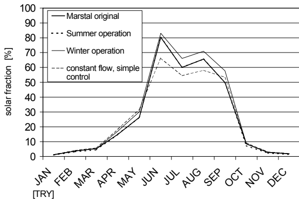
Figure 2. Comparison of the monthly solar fraction for different control strategies and the second generation plant (Marstal case).
