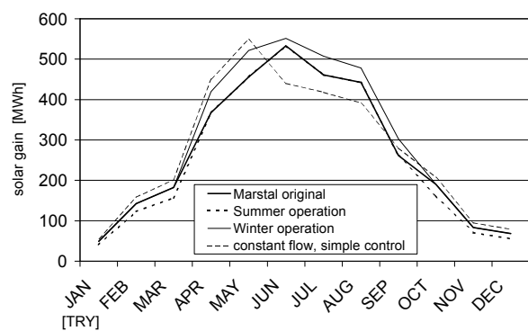
Figure 1. Comparison of the monthly solar gain for different control strategies and the second generation plant (Marstal case).
