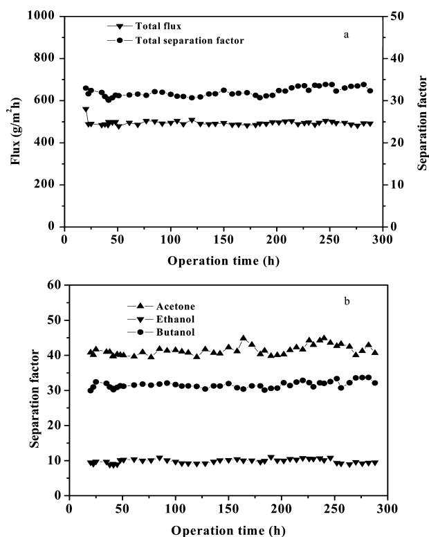
Figure 8. Pervaporation performance of the silicalite-1 filled PDMS/PAN composite membrane in continuous ABE fermentation–PV coupled process; D = 0.0117 \text{ h}^{-1} .
