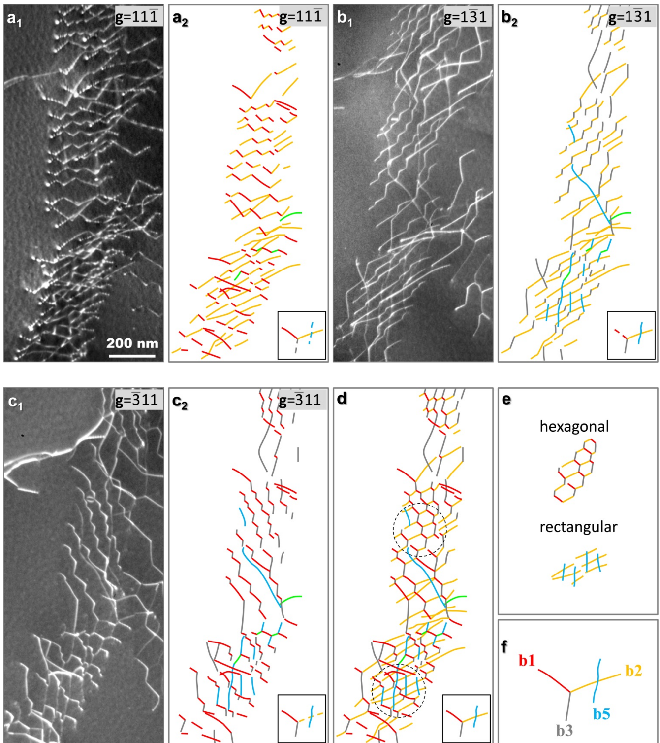
Figure 5 Determination of dislocation content of GNB2. (a 1 ,b 1 ,c 1 ) Example weak-beam images using g=[11\bar{1}] , g=[1\bar{3}1] and g=[\bar{3}11] , respectively. (a 2 ,b 2 ,c 2 ) Tracings of visible dislocations of (a 1 ), (b 1 ) and
