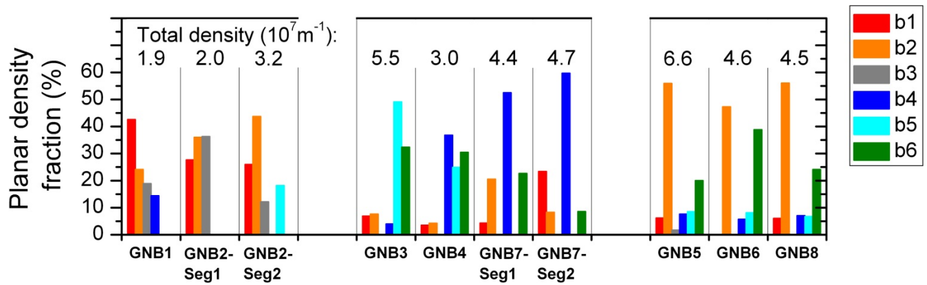
Figure 11 Planar dislocation densities of the GNBs corresponding to Fig. 10. For each GNB segment, the total planar dislocation density is indicated, and the fraction of each set of dislocations within the boundary is plotted.
