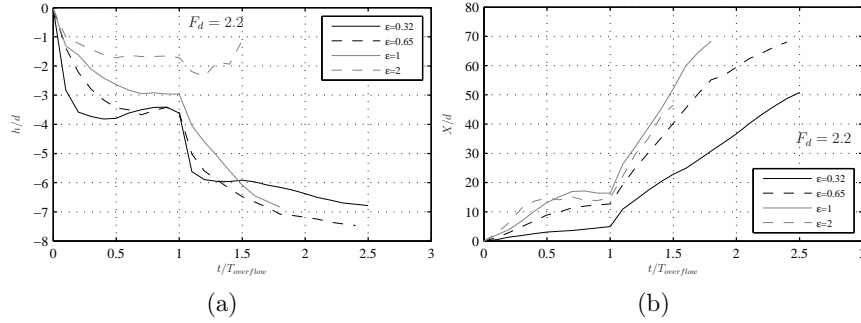
FIG. 10: Time-series of the vertical (a) and horizontal (b) position of the centroid of the plume, normalized with the overflow pipe diameter d . T_{overflow} represents the time when the overflow discharge stops.
