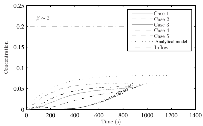
FIG. 7: Overflow concentrations until the bed level inside the hopper is 80%
