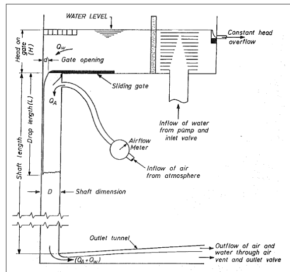
FIG. 2: Experimental setup of Whillock and Thorn (1973)
