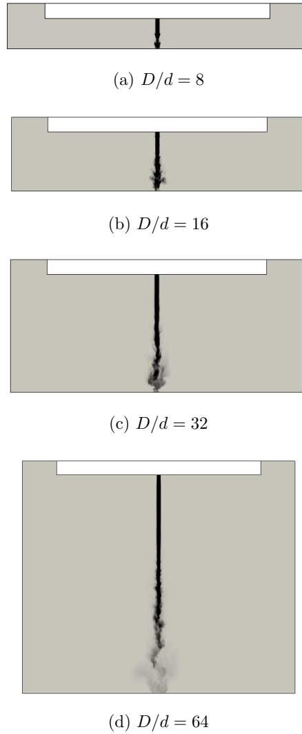
FIG. 13: Overflow buoyant jet under calm water condition ( \epsilon = 0 , F_d = 2.2 ), in different depths
