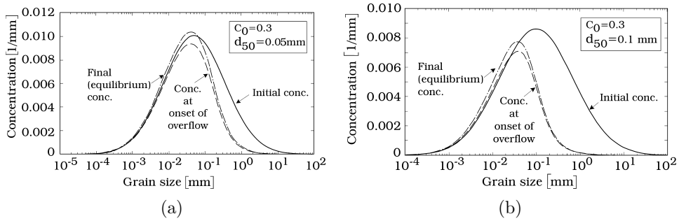
FIG. 11: Inflow concentrations, concentrations at the onset of overflow, and concentrations at equilibrium with \sigma = 7 ; (a) \bar{\beta} = 0.2 ; (b) \bar{\beta} = 3.0
