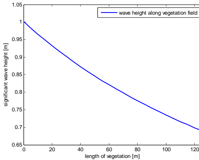
Figure 5 Wave height change for full vegetation
