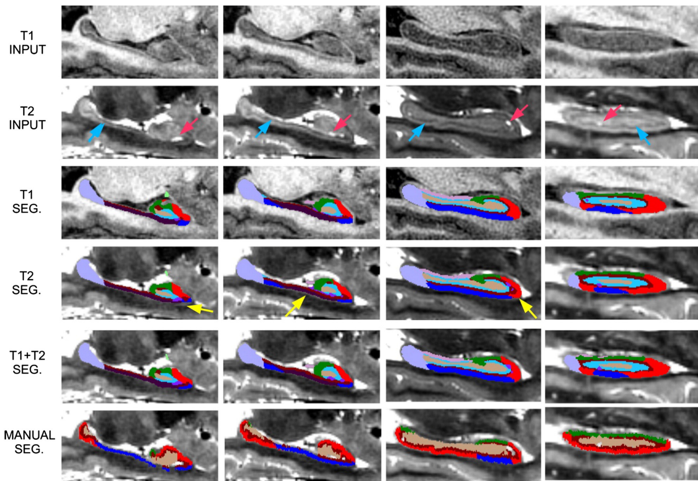
Fig. 9. Sample sagittal slices of “subject 3” from Winterburn et al. (2013), from medial (left) to lateral (right). See caption of Fig. 8 for an explanation of the different rows. The red arrow marks a CSF pocket, the blue arrows mark the molecular layer, and the yellow arrows mark segmentation errors in the whole hippocampal shape.
