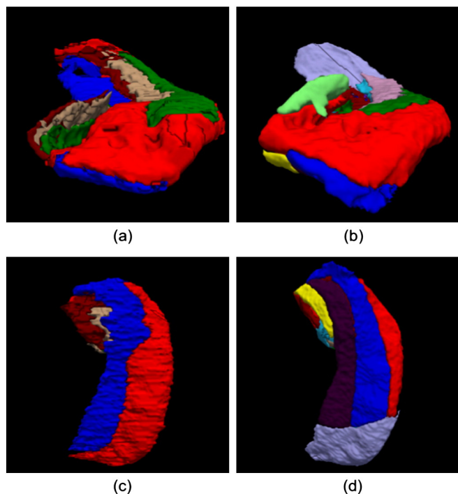
Fig. 10. 3D renderings of segmentations of the high-resolution T1/T2 data. (a) Manual segmentation from Winterburn et al. (2013), anterior view. (b) Automated segmentation using T1 and T2 volume simultaneously, anterior view. (c–d) Inferior view of (a–b).
