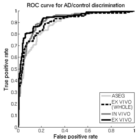
Fig. 13. ROC curves for the AD discrimination task using a LDA classifier on the hippocampal subregion volumes estimated by the ex vivo atlas (FreeSurfer v6.0) and the in vivo atlas (FreeSurfer v5.3 and earlier), as well as for discrimination based on whole hippocampal volume as estimated by FreeSurfer ("aseg") and by the ex vivo atlas (adding up the volumes of the subregions).
