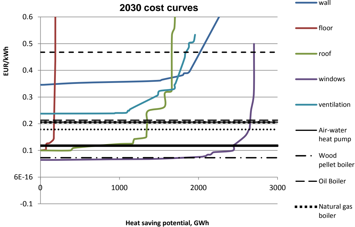
Figure 5 Heat saving and heat generation marginal cost curve for 2030.
