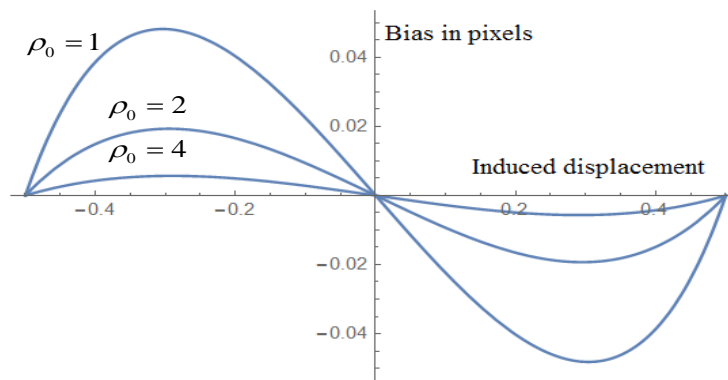
Fig.3. The bias effect for varying the induced displacement from -0.5 to 0.5 pixels for three values of the speckle size \rho_0 . The array parameters are \Lambda = 1 , \omega_0 = 1000 and \omega_p = 0.7 .
