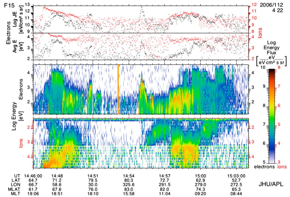
Figure 10. (first panel–fourth panel) Data from the DMSP F15 particle spectrometers. The energy fluxes of the electrons and ions are plotted for the interval 14:46–15:04 UT, with color codes in Figure 10 (third and fourth panels), along with the ion and electron integral energy flux and average energy. The orange line in Figure 10 (third panel) represents the time when DMSP F15 passed directly above NRD.
