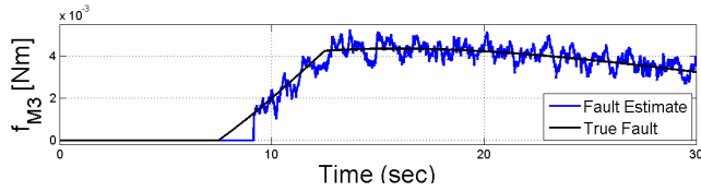
Fig. 7. Estimate of the actuator fault F_{M_3} .
