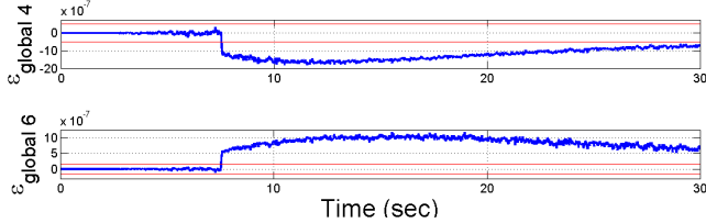
Fig. 5. Sensor fault scenario: decoupled global residuals sensitive to the actuator fault f_{M_3} with constant gain.
