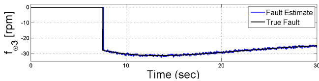
Fig. 8. Estimate of the physical sensor fault F_{\omega_3} .
