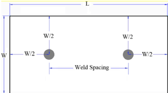
Fig. 3 Geometrical Details of Test Coupons.
