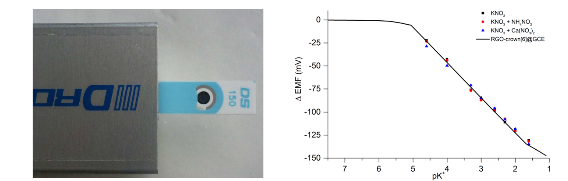
a) Picture of disposable SPE with RGO-crown[6] dropcast. b) Response of potential on SPE@RGO-crown[6] from different samples containing K^+ either as pure solution or "polluted" with 10 mM NH_4^+ or 5 mM Ca^{2+} .
