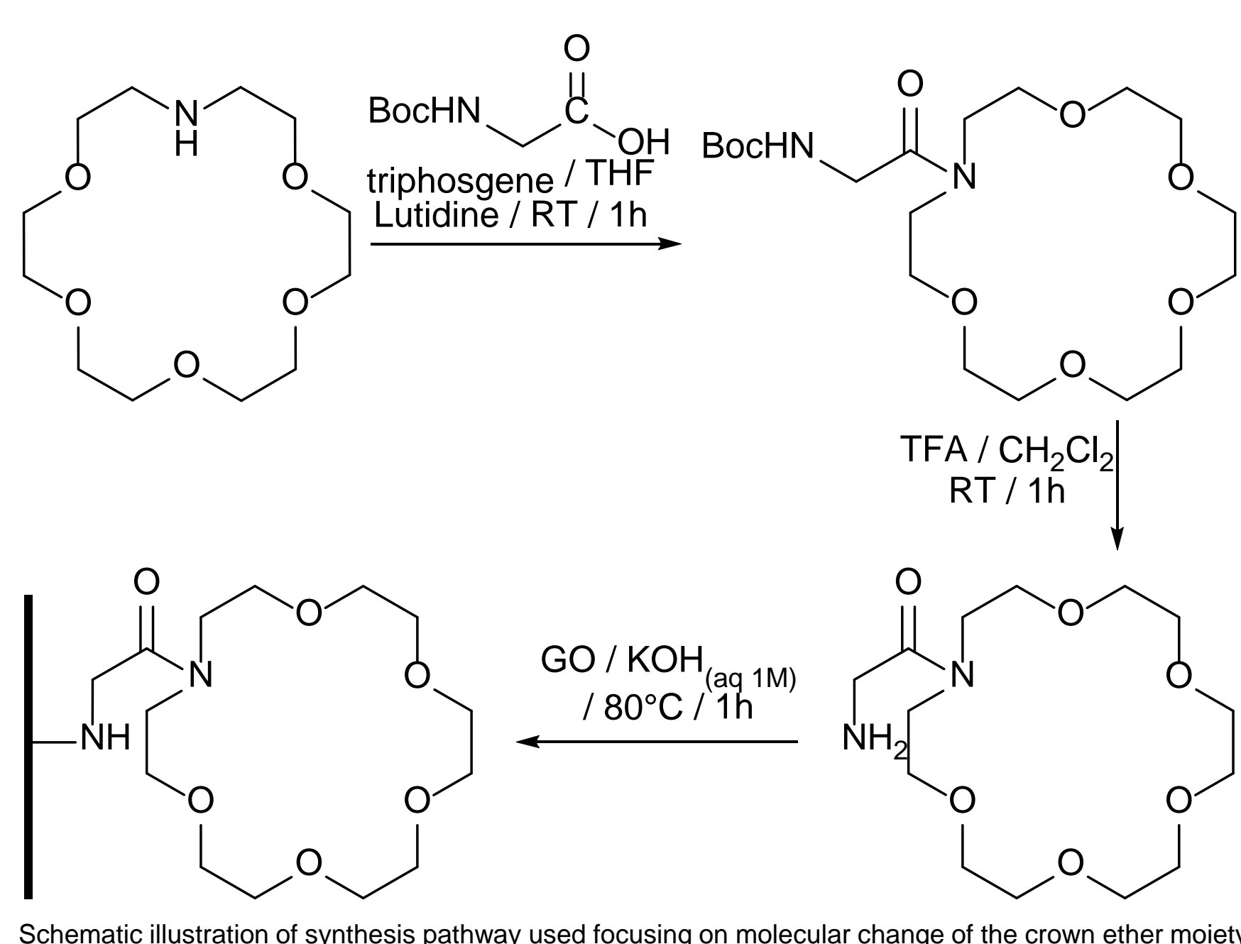
Schematic illustration of synthesis pathway used focusing on molecular change of the crown ether moiety
