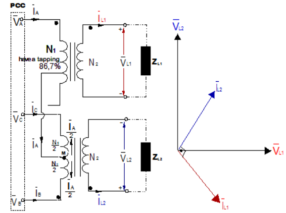
Figure 3-2: Scott connection and its phasor diagram [4][5]
