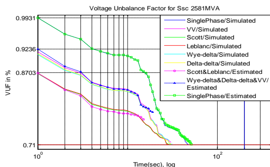
Figure 6-4: VUF (%) for different type of transformers obtained by Simulations and Estimation Formulas (+7.5% corrected)
