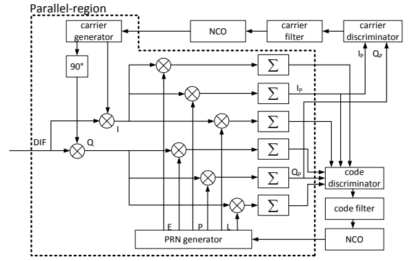
Figure 7: Tracking loops for one channel
