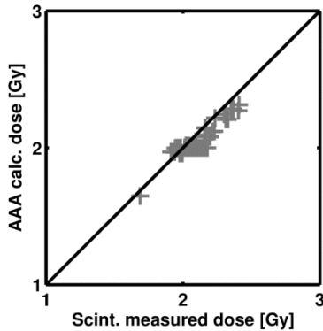
Figure 36. The AAA calculated dose relative to the scintillator measured dose. If the markers are situated exactly on the black line there is no difference between the doses. AAA calculates a lower dose compared to the scintillator measurements if the markers are situated below the black line.
