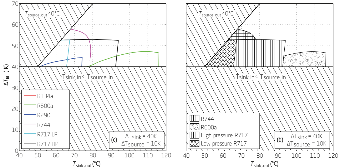
Figure 38 - Working domains of single-stage heat pumps.
