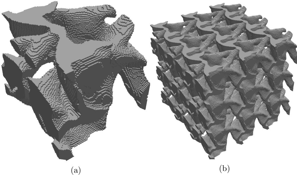
Figure 4: 3D isotropic microstructure with Poisson's ratio -0.51 . a = 0.125\% is used for the stiffness constraint on the eroded design, while the isotropy constraint parameter \epsilon is set to 10^{-5} for all three designs. The solid volume fraction of the dilated design is constrained to 40%. The initial guess is a random distribution of densities. (a) One unit cell. (b) 3 \times 3 \times 3 unit cells.
