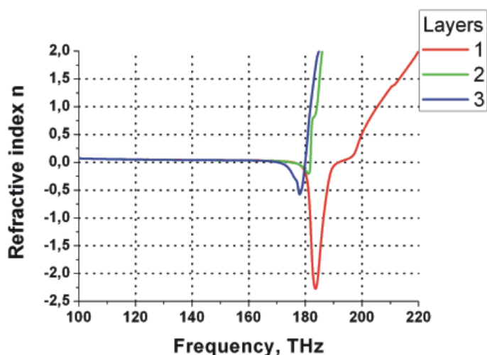
FIG. 12 Retrieved refractive index for one (red), two (green) and three (blue) layers of SCiC
