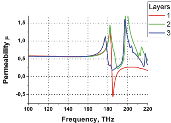
FIG. 13 Retrieved permeability for one (red), two (green) and three (blue) layers of SCiC
