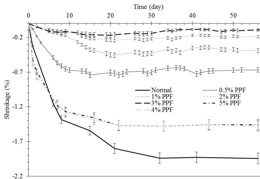
Fig 9. PPF content effect on controlling the shrinkage of fly ash based geopolymer.
