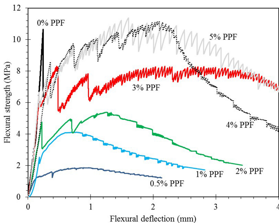
Fig 12. Flexural strength-deflection curve of PPF geopolymer matrix at 56 days.
