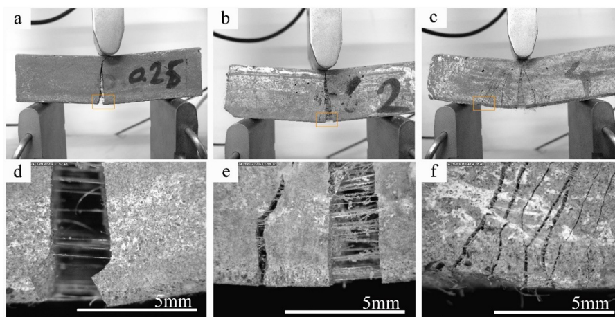
Fig 14. Fracture mode and toughening mechanism of PPF reinforced fly ash based geopolymer.
