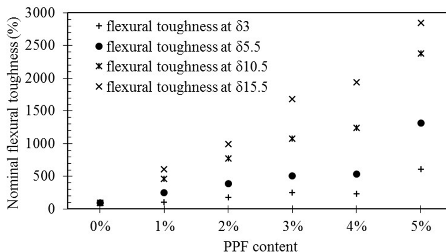
Fig 13. Nominal flexural toughness improvement of PPF fly ash based geopolymer composites at 56 days.
