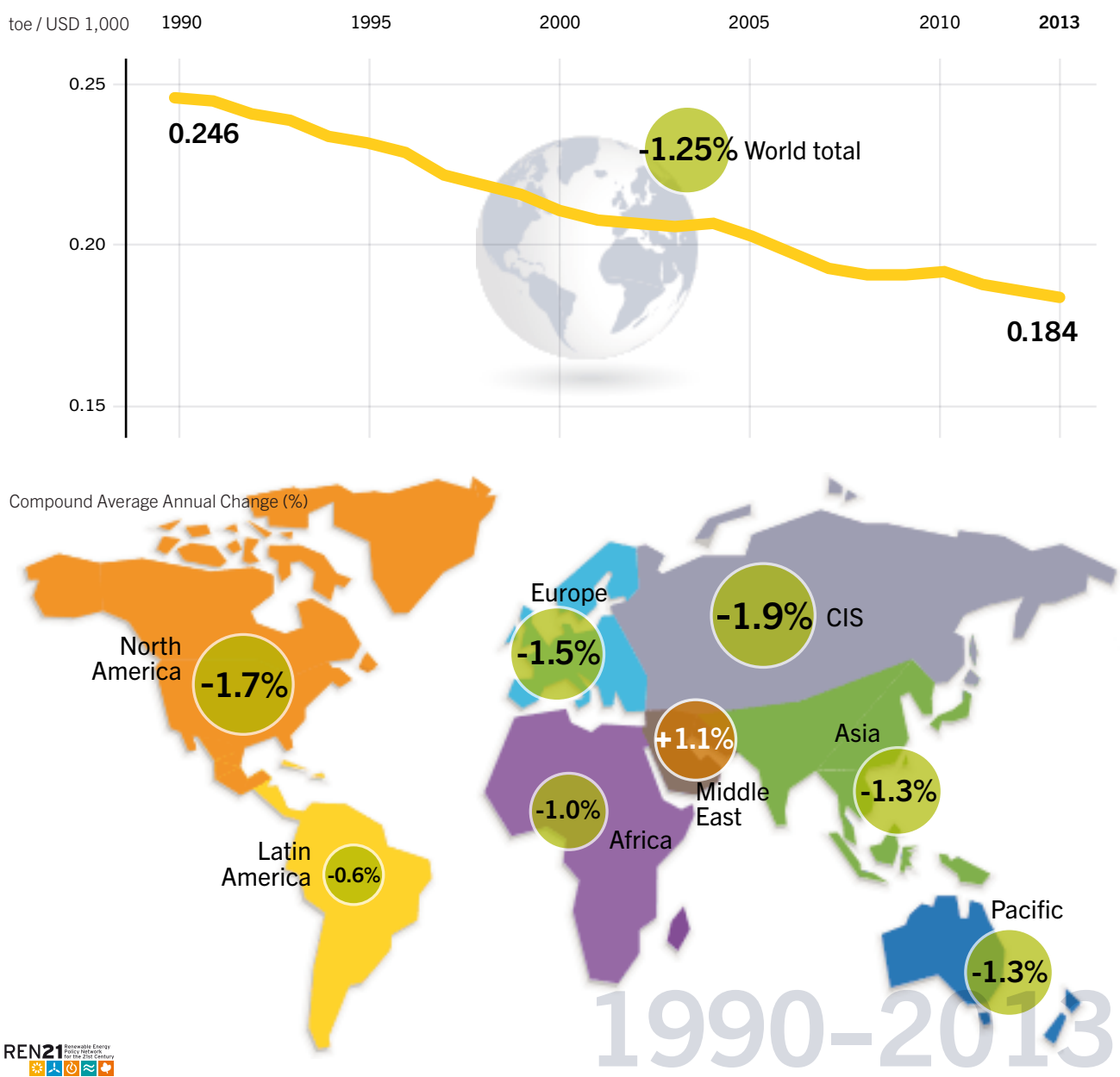
Figure 37. Global Energy Intensity, 1990–2013
