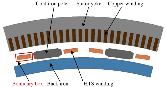
Fig. 2. Illustration of a pole pair segment in a 2-MW partially HTS wind generator. The red rectangle represents the coupling boundary of the machine model and the ac loss model.
