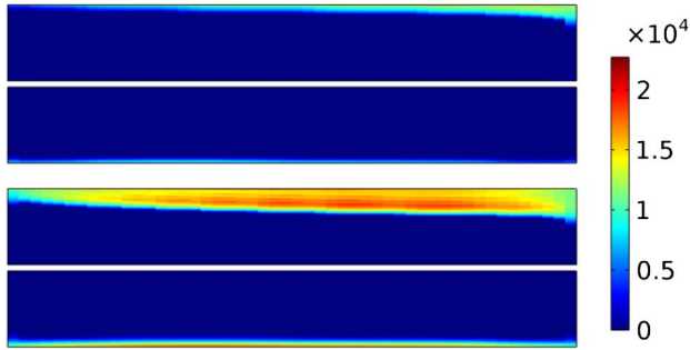
Fig. 5. The distributions of the ac loss density Q_{ac} ( W/m^3 ) for half of an HTS winding at t = 60 s (upper) and t = 120 s (lower).
