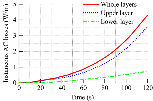
Fig. 6. Instantaneous ac losses for the upper HTS layer, lower HTS layer, and the whole layers. Note that only half of an HTS winding is considered; hence, the values shown here should be doubled to evaluate the actual ac losses in a full HTS winding.
