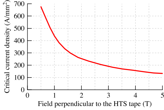
Fig. 3. Field dependence of the critical current density for AMSC's Amperium 12-mm HTS tape operating at 30 K. The tape has a critical current of 350 A at 77 K, self-field.
