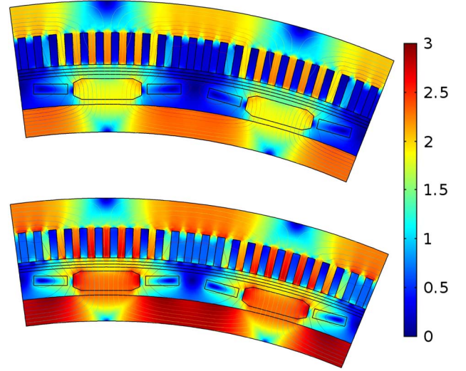
Fig. 4. The magnetic field distributions in the machine at t = 60 s (upper) and t = 120 s (lower). The current in the HTS winding is ramped up from 0 to 480 A at a constant rate of 4 A/s.
