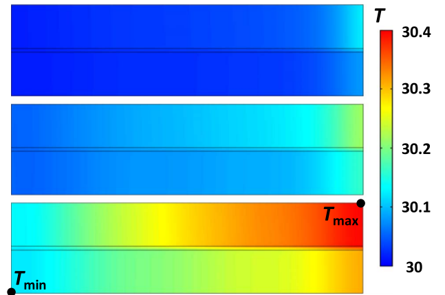
Fig. 7. The temperature distribution for half of an HTS winding at t = 60 s (upper), t = 90 s (middle), and t = 120 s (lower). T_{max} and T_{min} are the points that have the maximum and minimum temperature rise, respectively.
