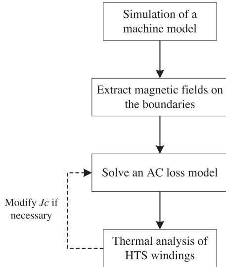
Fig. 1. Flowchart of the modeling strategy to compute ac losses and their thermal effect in an HTS machine.
