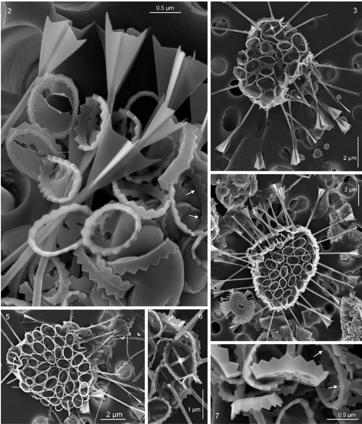
Figs 2–7. Papposphaera heldalii SEM images of cells from the Svalbard region collected during Jan. 2014 (Figs 4–5) and March 2014 (Figs 2–3, 6–7). 2 – cluster of coccoliths shown at high magnification. Notice in particular details of the calyx and coccolith rim calcification. The arrows point to extensions from the pentagonal elements separating the rod-like elements. See also ruptures in the organic base plates of body coccoliths; 3 – whole cell (type specimen) showing the general disposition of types of coccoliths within the coccosphere. A single coccolith (enlarged in Fig. 6) shows the central area calcification of a calicate coccolith; 4 – whole cell. Notice the difference in length of the central process among the two clusters of coccoliths carrying these. See also the conspicuous size differences between neighboring body coccoliths; 5 – body coccoliths showing large individual size differences; 6 – detail of central area calcification in a coccolith that carries a central process (broken away here); 7 – detail of coccolith rim from coccoliths that carry a central process. The arrows point to extensions from the pentagonal elements separating the rod-like elements.
