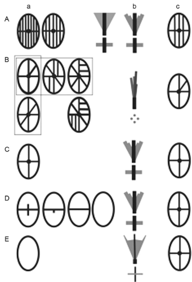
Fig. 8. Schematic drawings of coccolith structures in species of Papposphaera (not drawn to scale). a – body coccoliths; b – calyx design; c – coccoliths with central processes; A – P. sagittifera ; B – P. sarion ; C – P. arctica ; D – P. iugifera ; E – P. heldalii . Notice that alternative shapes are included for some species (A/a, B/a, D/a) and that the P. sarion design for a coccolith with a central process (B/c) is potentially as variable as B/a.
