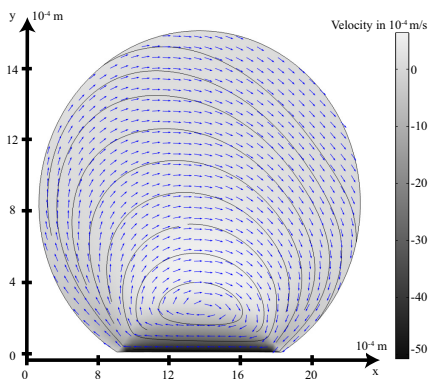
Fig. 11. A drop with \theta = 160^\circ , and \Delta\theta = 10^\circ on an incline of \alpha = 1^\circ . The drop is depicted in the centre of mass frame of reference, moving to the right. The velocity field directions indicated by normalised arrows and the streamlines and contour plot shows the size of the velocity. The simulation time is t = 0.045 s.
