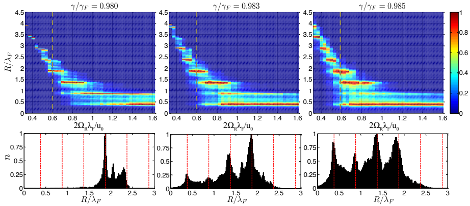
Figure 8.19: Numerical simulations showing the dependence of the orbital statistics on the dimensionless rotation rate 2\Omega_R\lambda_F/u_0 , for three different values of memory \gamma/\gamma_F . Each simulation was performed with rest initial conditions, with \Delta t = 2^{-8} and t_{\max} = 1000 . In the top panels, each column is colored according to the prevalence of the corresponding loop radius R , with red segments corresponding to the most prevalent radii. The bottom panels show three sample probability distributions at 2\Omega_R\lambda_F/u_0 = 0.6 . The peaks of the probability distributions are centered around the zeros of the Bessel function J_0(k_F r) , indicated by the red dashed lines.
