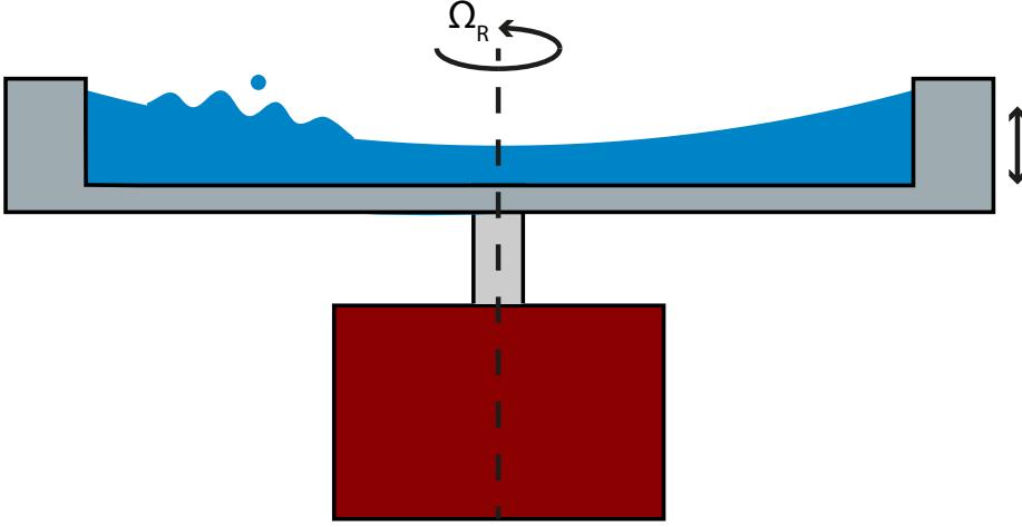
Figure 8.1: The experimental set-up. The fluid bath is vibrated vertically and rotated around an vertical axis at the center of the bath. The rotation rate about the centerline is denoted \boldsymbol{\Omega}_R = \Omega_R \hat{\mathbf{z}} .
