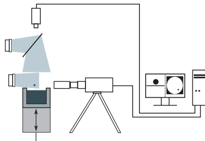
FIG. 2. Schematic illustration of the experimental set-up. The vibrating bath is illuminated by two LED lamps, and the drop motion recorded by two digital video cameras. The top view camera captures images at 17.5–20 frames per second, while the side view camera records at 4000 frames per second. The video processing is done on a computer.
