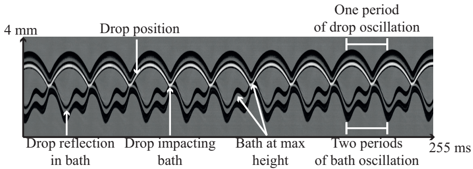
Figure 7.2: Spatio-temporal diagram of a (2,1) mode with interpretative arrows showing the drop reflection in the bath, the drop position, the drop impacting the bath, the math positions of max height of the bath, and finally the periods of the drop and bath oscillations, respectively.
