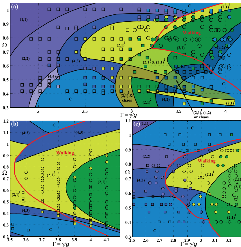
FIG. 3. Regime diagrams indicating the dependence of the droplet behaviour on the dimensionless driving acceleration, \Gamma = \gamma/g , and the vibration number, \Omega = 2\pi f \sqrt{\rho l_0^3/\sigma} . (a) The 20 cS-80 Hz combination, for which \Gamma_F = 4.22 \pm 0.05 . (b) The 50 cS-50 Hz combination, for which \Gamma_F = 4.23 \pm 0.05 . (c) The 20 cS-70 Hz combination, for which \Gamma_F = 3.33 \pm 0.05 . Coloured areas correspond to theoretical predictions, the solid red line denoting the theoretically predicted walking threshold. Experimental data are presented as square or round markers, with square markers denoting stationary bouncing states, round markers walking states, and their colour indicating the associated mode.
