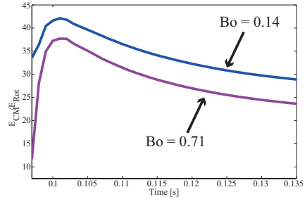
Fig. 9. The fraction \frac{E_{CM}}{E_R} as a function of time for increasing Bond number. The inclination is \alpha = 1^\circ , the contact angle is 140^\circ and the surface is tilted at t = 0.1 s.
