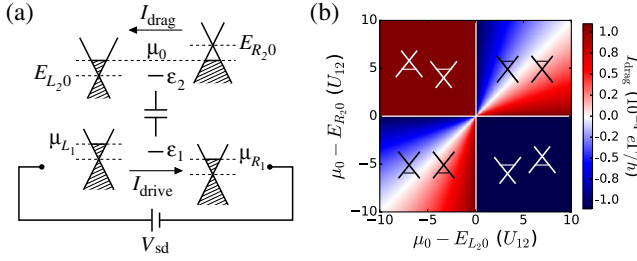
FIG. 3. (a) Energy level diagram of the graphene-based CQD in Fig. 1(c). The QD levels, \epsilon_i = -eV_i , and the positions of the Dirac points in the leads, E_{\alpha 0} = -eV_{\alpha} , are controlled by local gates. (b) Drag current as a function of gate voltage on the leads of the drag system (see Dirac cone insets) at the upper triple point in the stability diagram. Parameters (in units of U_{12} ): U_{12} = 1 , \Gamma_{L10/R10} = 0.01 \equiv \Gamma , \Gamma_{L20/R20} \propto |\mu_0 - E_{L20/R20}| , \partial\Gamma_{L2/R2} = \text{sgn}(\mu_0 - E_{L20/R20}) , t_{L2} = t_{R2} , eV_{sd} = 0.1 , k_B T = 0.01 .
