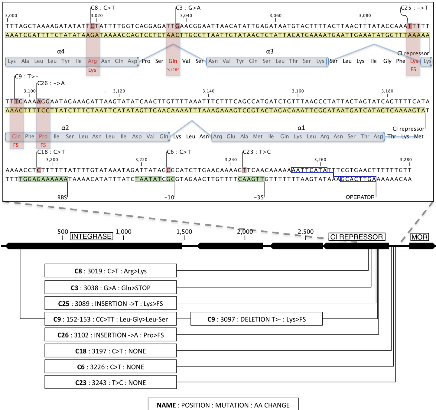
Fig 1. Localization of TP901-BC1034 clear plaque mutations. Expanded view of the region from position 0 to 3600 showing the clear plaque mutations. A physical map of orf1 (Integrase) to orf5 (Mor) is shown in the middle with a size indicator. Below this each mutation is identified in boxes according to its [designation: precise position: nucleotide change: change at the amino acid level (STOP = nonsense mutation; FS = frameshift mutation; NONE = no change in amino acid sequence)]. Above the physical map is a panel showing the genetic context of the CI mutations. Below the nucleotide sequence the amino acid sequence is indicated with boxing of amino acids that are believed to form alpha helical structures (alpha1 to alpha4) in the wild type CI protein [5]. Extended promoter -10 and -35 elements and the ribosomal binding site (RBS) are highlighted in green. The O_R site is indicated in blue box (operator). The O_L site is located 63 bp further to the right of the O_R site overlapping the start of the O_L transcript (not shown).
