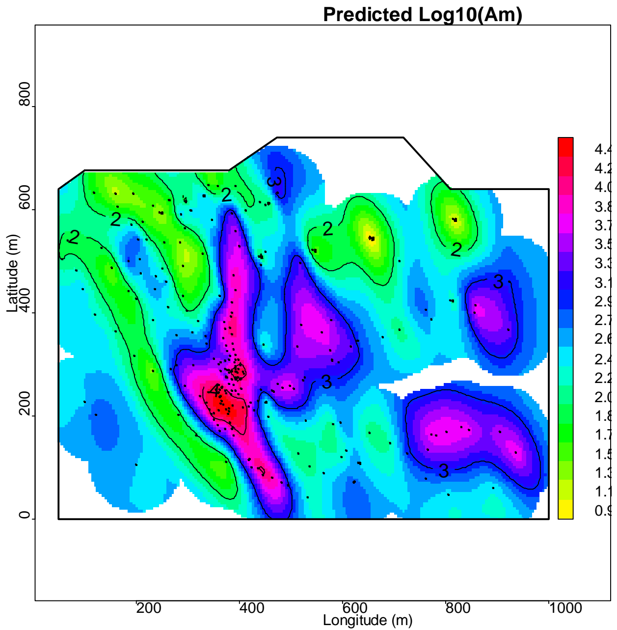
Figure 50 Spatial prediction of the \text{log}_{10}(A_m) concentration in sub-region 2. Model with Anisotropy. Black dots are measurement locations.
