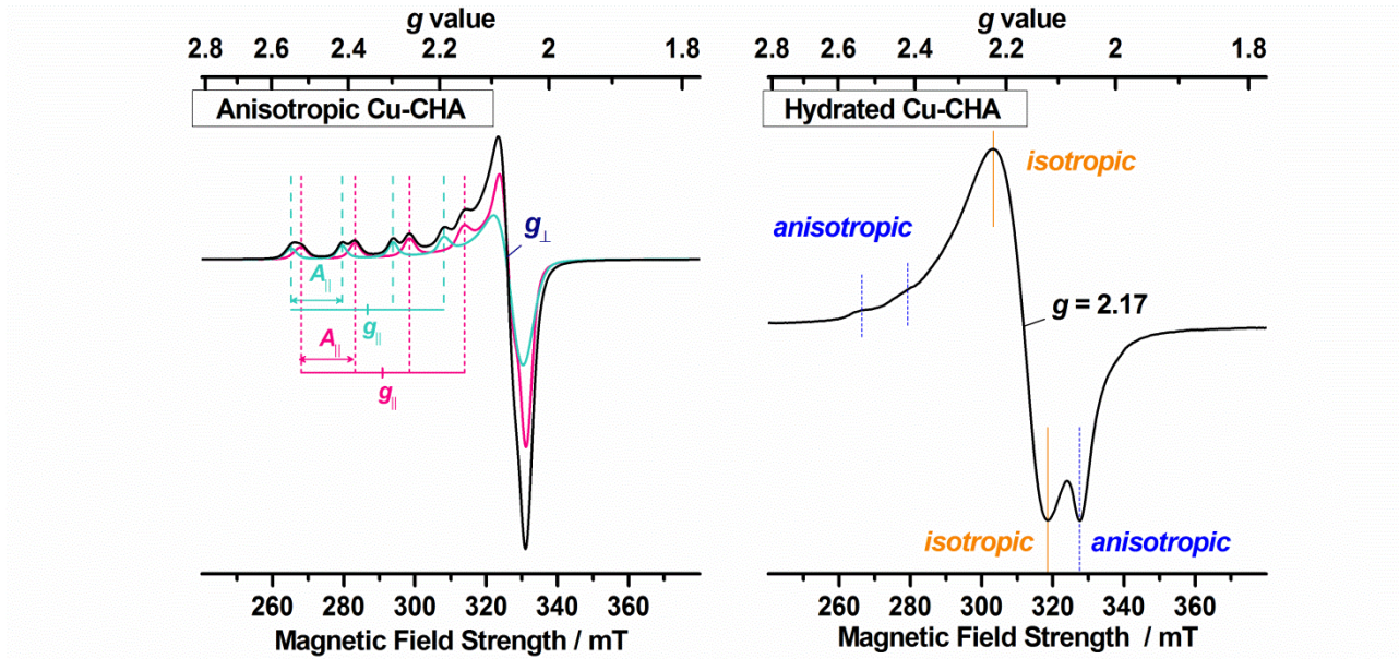
Fig. 1 Left: Calculated anisotropic spectrum (black) for two monomeric \text{Cu}^{2+} species with the parameters found for EPR signal 1 and 2 in a dehydrated Cu-CHA sample. The spectrum is found as a simple sum of the spectra for each species, which are shown in pink for signal 1 and in teal for signal 2. The values used in the simulation are given in Table 1. The characteristic splitting of the line centered at g_{\parallel} due to the interaction with the copper nucleus is indicated for each species. Right: Experimental spectrum obtained at room temperature
