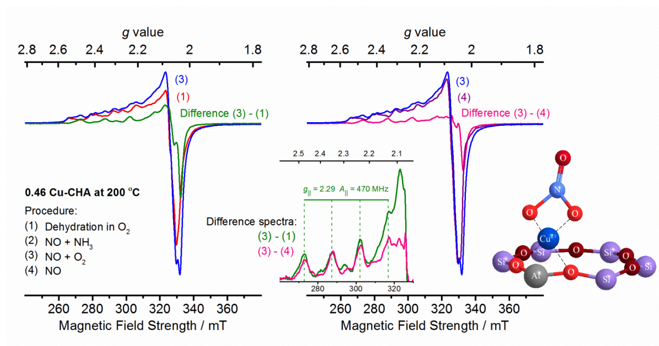
Fig. 5 In-situ X-band EPR spectra at 200 °C of Cu-CHA (Si/Al = 14, Cu/Al = 0.46) exposed to SCR relevant gas mixtures [8]. Left : Experimental EPR spectra obtained at 200 °C after dehydration of the sample for 2 h in a flow of O 2 /He at 250 °C (red trace, spectrum 1). The same sample was then exposed to a flow of (200 mL/min) of NO (1000 ppm), NH 3 (1200 ppm) and balance He for 20 min followed by a flow of NO (1000 ppm) and O 2 (10 %) and balance He until steady state (blue trace, spectrum 3). The difference spectrum (green trace) is obtained by simple subtraction of the red spectrum from the blue in every point. Middle : The same sample was then exposed to a flow of NO (1000 ppm) and balance He (purple trace, spectrum 4). The difference spectrum between spectrum 3 and spectrum 4 is shown as the pink trace. Details of the difference spectrum from the left panel, (3)-(1) and from the middle panel, (3)-(4) are plotted for comparison in the insert in the middle panel. Right : Suggested structure for the bidentate nitrate [8, 39].
