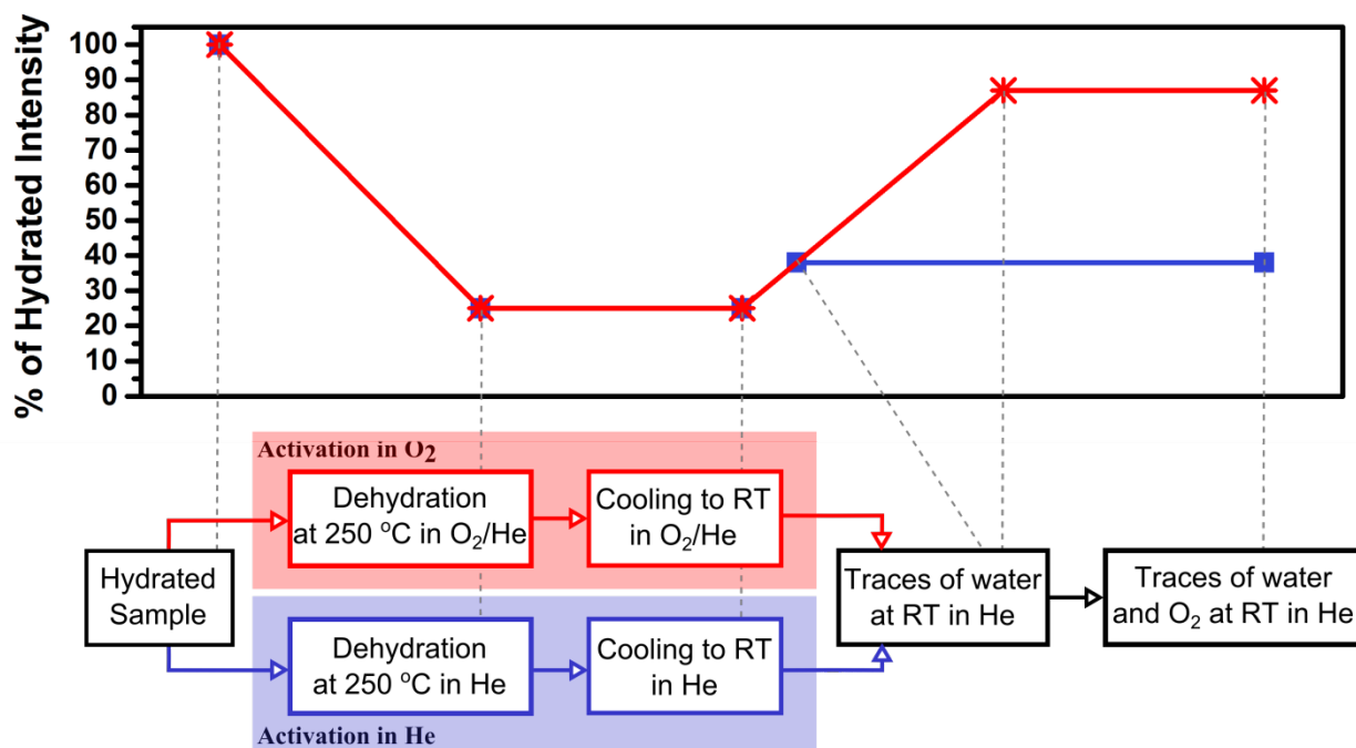
Fig. 4 Bottom: Graphical representation of the in-situ EPR procedure performed while monitoring with EPR. The O 2 activation procedure (upper path, red) took place in 20% O 2 and balance He, the other in pure He (lower path, blue) [12]. Top: EPR signal intensity corresponding to the sample having equilibrated under the gas flows given below, where the stars and the red line correspond to the O 2 activation and the squares and the blue line to the He activation. Both were performed with a flow of 100 mL/min on 20 mg of two identical fractioned (150 – 300 \mu\text{m} ) Cu-CHA samples with Si/Al = 14 and Cu/Al = 0.46. The intensity at 250 °C has been corrected with the Boltzmann equation to be comparable with the intensity at RT.
