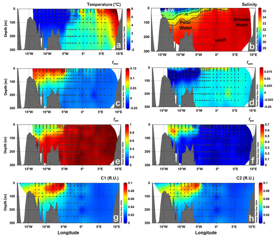
Figure 3. Vertical sections across the surface layer of Fram Strait in September 2013. (a) temperature (°C), (b) salinity, fractions of (c) meteoric water ( f_{mw} ), (d) sea-ice melt ( f_{sim} ), (e) Atlantic water ( f_{aw} ) and (f) Pacific water ( f_{pw} ), (g) C1 (R.U.) and (h) C2 (R.U.). In (b) black lines indicate the potential density ( \sigma , \text{kg m}^{-3} ) and the abbreviations indicate the position of the water masses defined based on T-S diagrams (Fig. 1). Produced with Ocean Data View 60 .
