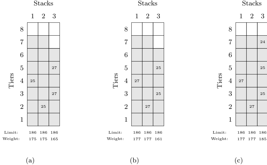
Figure 5: Exchanging containers between stacks
