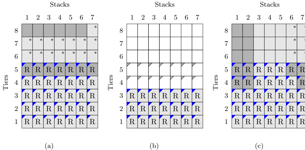
Figure 3: Improving solutions. Removing last containers stowed
