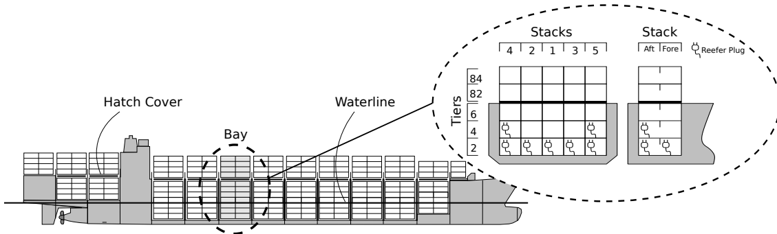
Figure 1: The layout of a container vessel
