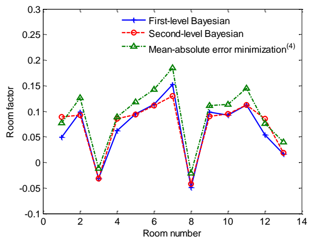
Figure 4 Comparison between the Bayesian-based room factors and the ones from the mean-absolute error minimization.
