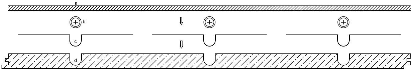
Figure 2. a) Floor covering b) Pipe, 17x2.0 mm c) Heat distribution plate, 0.3 mm, d) Under-floor plate, 22 mm
