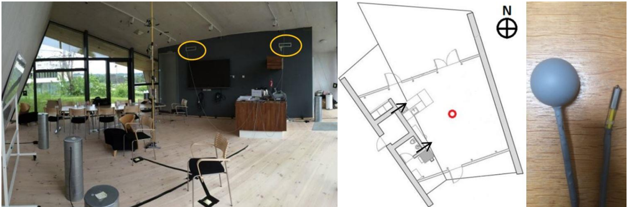
Figure 3. Panoramic view of the interior (left), the measurement location (middle) and the globe and air temperature sensors (right)
