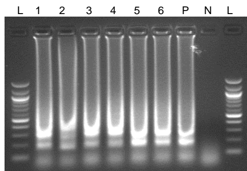
Fig. 3 Test of inhibitory effect of magnetic beads on LAMP reaction. 20 \mu l, 50 \mu l, 80 \mu l, 100 \mu l, 150 \mu l and 200 \mu l of Dynabeads® solution were centrifuged at 5000 \times g for 5 min and washed three times with sterile water. After washing, 10 \mu l of LAMP master mixture and 1 \mu l of 2 ng/ \mu l Salmonella DNA were added into the tubes and LAMP was performed at 65 °C for 40 min and terminated the reaction at 80 °C for 2 min. L: ladder; lane 1: 200 \mu l; lane 2: 150 \mu l; lane 3: 100 \mu l; lane 4: 80 \mu l; lane 5: 50 \mu l; lane 6: 20 \mu l; P: positive control; N: negative control.
