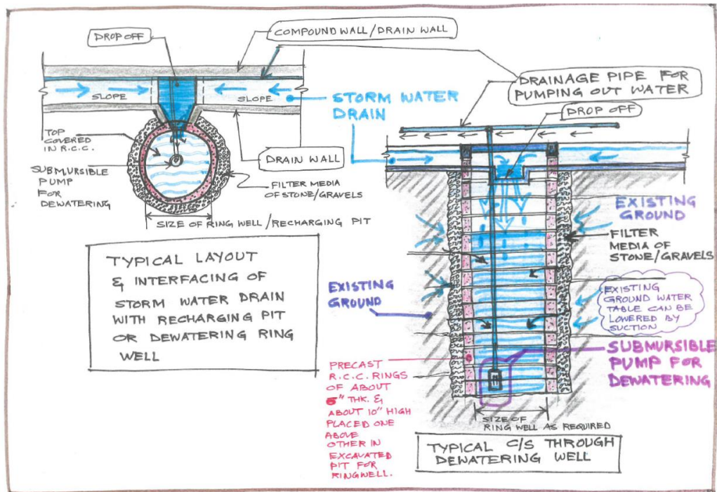
Figure A3: Structural adaptation measure – Surface storm water drainage and dewatering ring wells.
