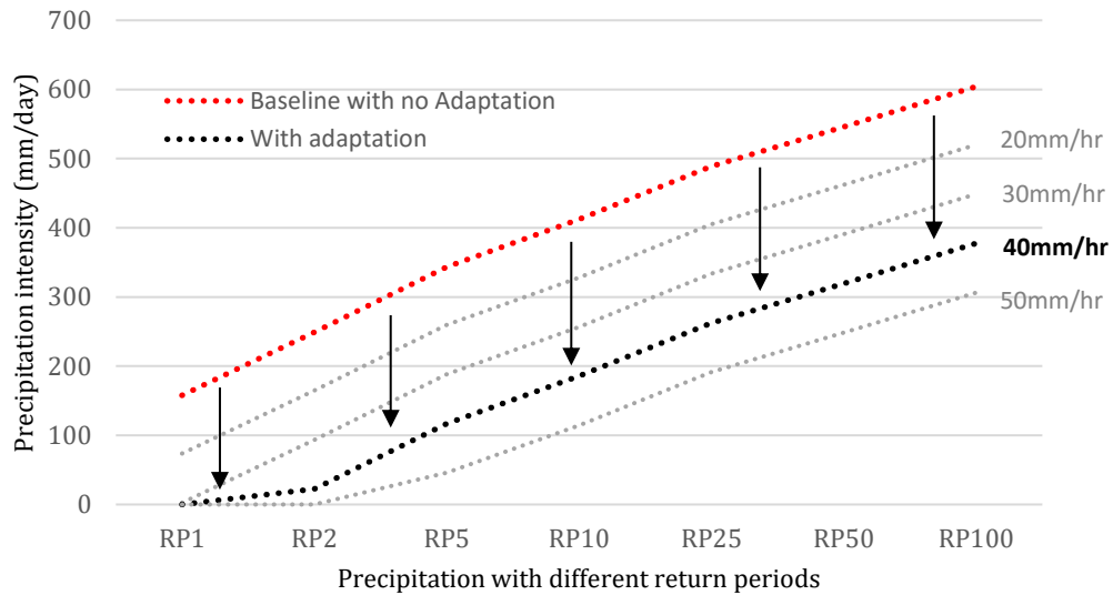
Figure 5. Precipitation potentially causing surface flooding and damages during extreme precipitation with different return periods (RP10 = 10 year return period) before and after implementation of structural adaptation measures with total protection levels of 20-50mm/hr. 20mm, 30mm, 40mm (included in the CBA) and 50mm are alternative water removal capacities related to the adaptation measures.
