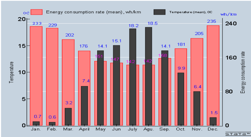
Figure 5.3.5: Mean ECR (in watt-hour per km) and the mean temperature (in °C) by month. The monthly mean ECR is presented on the y-axis to the right and the monthly mean temperature recorded during the trips is presented on the y-axis to the left.
