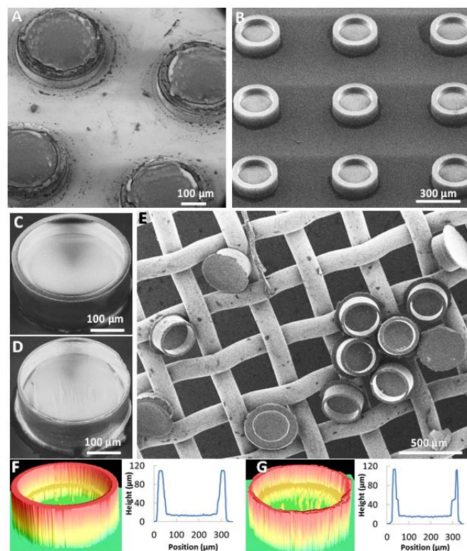
Figure 3 A. Punched microcontainers attached to Ni stamp after demolding, B. Microcontainers with 40 μm wall thicknesses bonded to the PAA-PEG sacrificial layer; C-D. Individual microcontainers with 20 μm (C) and 10 μm (D) wall thicknesses; E. Microcontainers filtered through a mesh after dissolution of PAA-PEG sacrificial layer; F. Height profile and 3D image of the microcontainers with 20 μm thick walls, G. Height profile and 3D image of the microcontainers with 10 μm thick walls. High aspect ratio of > 9 and wall heights of 120 μm are achieved.
