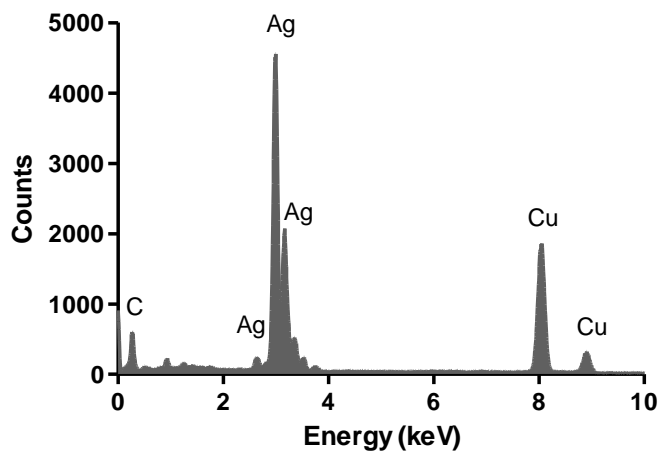
Figure 3: EDS spectrum for The Original Always Fresh Containers™ migration sample after 10 days in 3% acetic acid (Particle shown in Figure 2 D).
