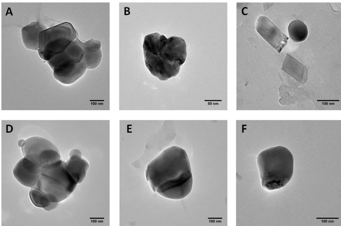
Figure 4: TEM results for migration solution samples after 10 days in 3% acetic acid. A and B: Fresher Longer™ Miracle Food Storage™ bags, C-F: Kinetic Go Green™ Premium Food Storage Containers. All the presented images were analyzed by EDS and confirmed the presence of titanium.
