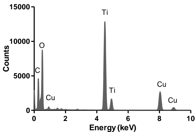
Figure 5: EDS spectrum for The Original Always Fresh Containers™ migration sample after 10 days in 3% acetic acid (Particle shown in Figure 4 D).
