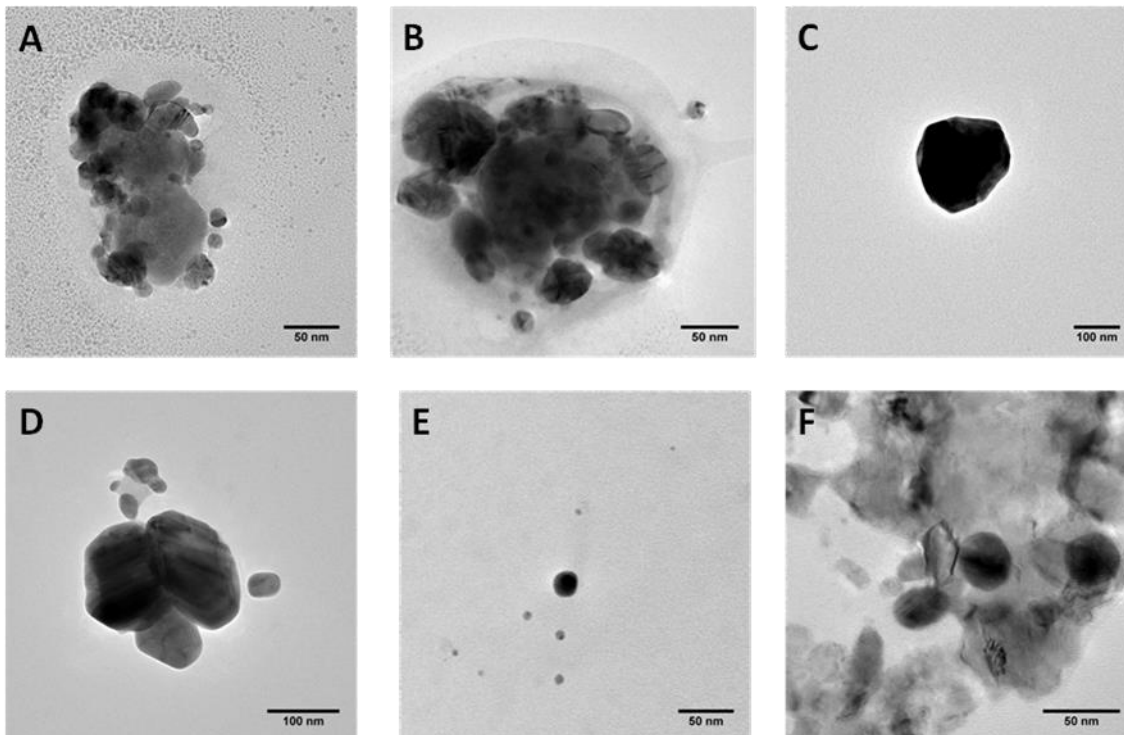
Figure 2: TEM results for migration solution samples after 10 days in 3% acetic acid. A: Fresher Longer™ Miracle Food Storage™ bags, B: Special Nanosilver Mother's milk pack, C and D: The Original Always Fresh Containers™, E and F: Kinetic Go Green™ Premium Food Storage Containers. All the presented images were analyzed by EDS and confirmed the presence of silver.
