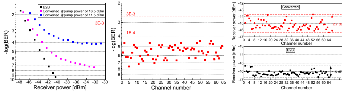
Fig. 3. Experimental results. Left: BER performance of one arbitrary tributary at pump power of 16.5 dBm and 11.5 dBm compared with B2B. Middle: BER performance of all 64 channels for pump power 16.5 dBm. Right: Receiver sensitivity at BER 3E-3 of all 64 converted channels (pump power 16.5 dBm) compared to B2B, yielding an average power penalty of 1 dB.
