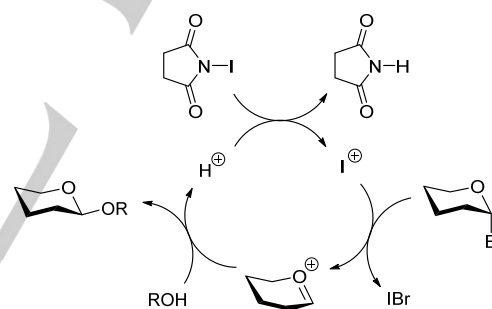
Scheme 2. Mechanism of the glycosylation reaction.
